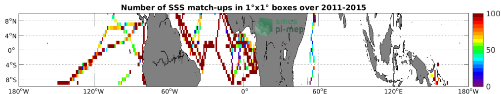
Figure 4: Number of SSS match-ups between TSG (GOSUD-Research-vessel) SSS and the Aquarius SSS L3 CAP v5 - 7-Day running (JPL) SSS product for the Equatorial Ocean 10N-10S Pi-MEP region over 1°x1° boxes and for the full satellite product period.
