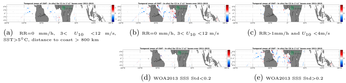
Figure 12: Temporal mean gridded over spatial boxes of size 1^\circ \times 1^\circ of \Delta SSS (Aquarius SSS L3 CAP v5 - 7-Day running (JPL) - TSG (GOSUD-Research-vessel)) for 5 different subdatasets corresponding to: RR=0 mm/h, 3 < U_{10} < 12 m/s, SST > 5^\circ\text{C} , distance to coast > 800 km (a), RR=0 mm/h, 3 < U_{10} < 12 m/s (b), RR > 1 mm/h and U_{10} < 4 m/s (c), WOA2013 SSS Std < 0.2 (d), WOA2013 SSS Std > 0.2 (e).
