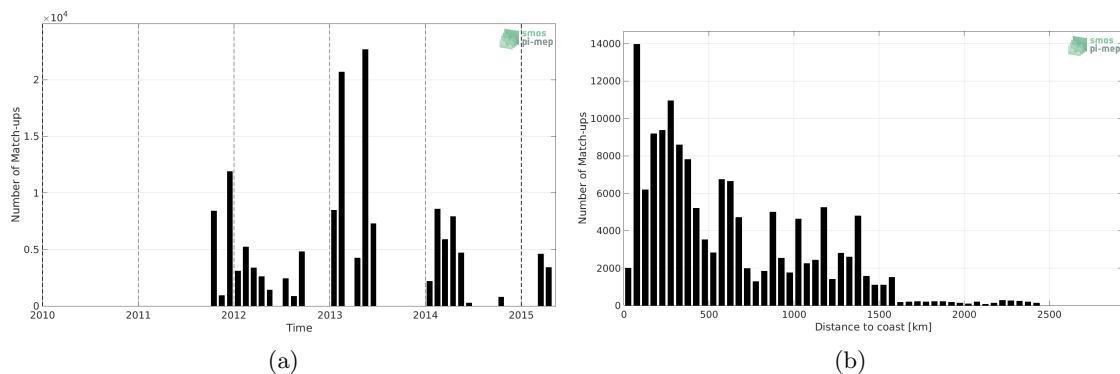
Figure 1: Number of match-ups between TSG (GOSUD-Research-vessel) and Aquarius SSS L3 CAP v5 - 7-Day running (JPL) SSS as a function of time (a) and as function of the distance to coast (b) over the Equatorial Ocean 10N-10S Pi-MEP region and for the full satellite product period.
