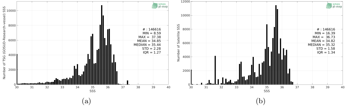
Figure 2: Histograms of SSS from TSG (GOSUD-Research-vessel) (a) and Aquarius SSS L3 CAP v5 - 7-Day running (JPL) (b) considering all match-up pairs per bins of 0.1 over the Equatorial Ocean 10N-10S Pi-MEP region and for the full satellite product period.
