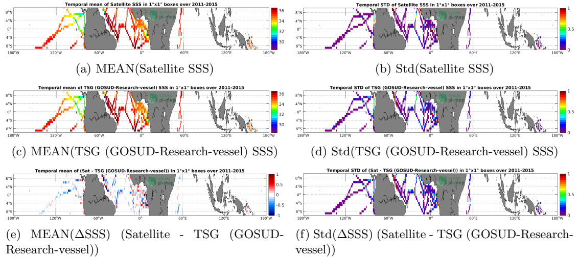
Figure 6: Temporal mean (left) and Std (right) of SSS from Aquarius SSS L3 CAP v5 - 7-Day running (JPL) (top), TSG (GOSUD-Research-vessel) (middle), and of \Delta SSS (Satellite - TSG (GOSUD-Research-vessel)). Only match-up pairs are used to generate these maps.
