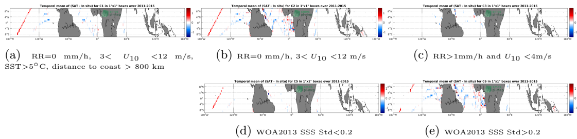
Figure 12: Temporal mean gridded over spatial boxes of size 1^\circ \times 1^\circ of \Delta SSS (Aquarius-L3-JPL-V5-7DAY-RUNNING - TSG-GOSUD-Research-vessel) for 5 different subdatasets corresponding to: RR=0 mm/h, 3 < U_{10} < 12 m/s, SST>5°C, distance to coast > 800 km (a), RR=0 mm/h, 3 < U_{10} < 12 m/s (b), RR>1mm/h and U_{10} < 4 m/s (c), WOA2013 SSS Std<0.2 (d), WOA2013 SSS Std>0.2 (e).
