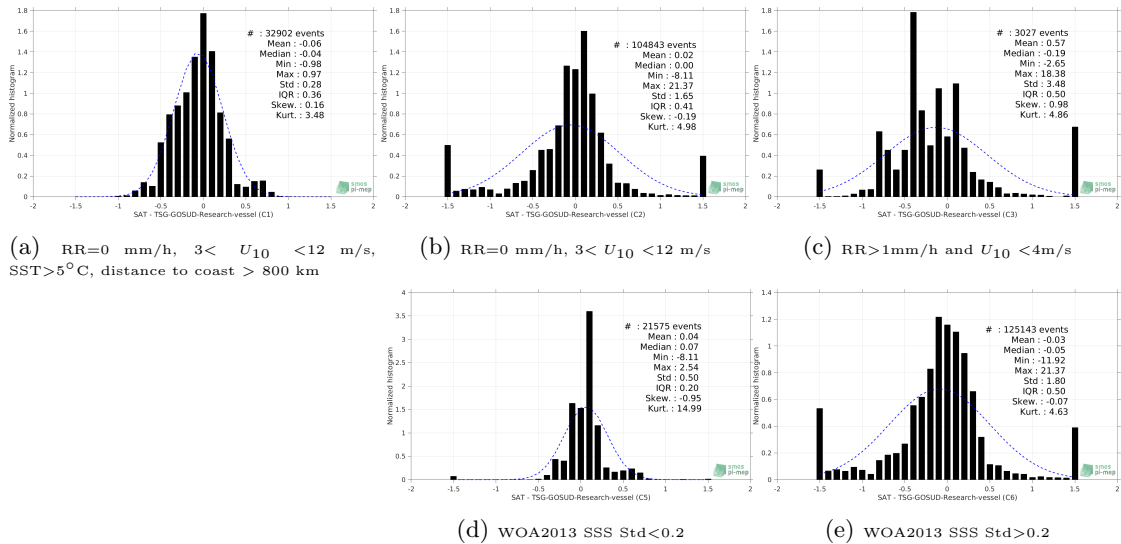
Figure 13: Normalized histogram of \Delta SSS (Aquarius-L3-JPL-V5-7DAY-RUNNING - TSG-GOSUD-Research-vessel) for 5 different subdatasets corresponding to: RR=0 mm/h, 3 < U_{10} < 12 m/s, SST>5°C, distance to coast > 800 km (a), RR=0 mm/h, 3 < U_{10} < 12 m/s (b), RR>1mm/h and U_{10} < 4 m/s (c), WOA2013 SSS Std<0.2 (d), WOA2013 SSS Std>0.2 (e).
