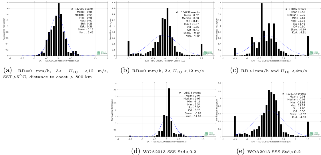
Figure 13: Normalized histogram of \Delta SSS (Aquarius-L3-JPL-V5-7DAY-RUNNING - TSG-GOSUD-Research-vessel) for 5 different subdatasets corresponding to: RR=0 mm/h, 3 < U_{10} < 12 m/s, SST >5^\circ C, distance to coast > 800 km (a), RR=0 mm/h, 3 < U_{10} < 12 m/s (b), RR >1 mm/h and U_{10} < 4 m/s (c), WOA2013 SSS Std <0.2 (d), WOA2013 SSS Std >0.2 (e).
