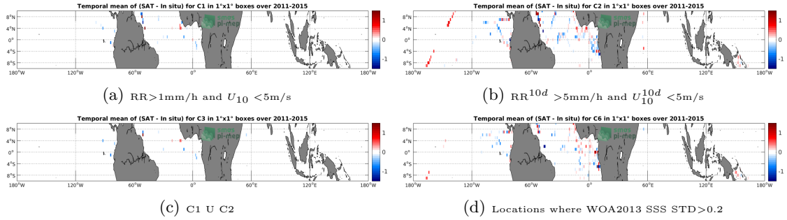
Figure 12: Temporal mean gridded over spatial boxes of size 1^\circ \times 1^\circ of \Delta SSS (Aquarius-L3-JPL-V5-7DAY-RUNNING - TSG-GOSUD-Research-vessel) for 4 different subdatasets corresponding to: RR > 1\text{mm/h} and U_{10} < 5\text{m/s} (a), RR^{10d} > 5\text{mm/h} and U_{10}^{10d} < 5\text{m/s} (b), C1 U C2 (c), Locations where WOA2013 SSS STD > 0.2 (d).
