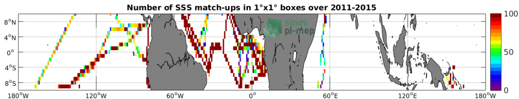
Figure 4: Number of SSS match-ups between TSG-GOSUD-Research-vessel SSS and the Aquarius-L3-JPL-V5-7DAY-RUNNING SSS product for the Equatorial Ocean 10N-10S Pi-MEP region over 1°x1° boxes and for the full satellite product period.
