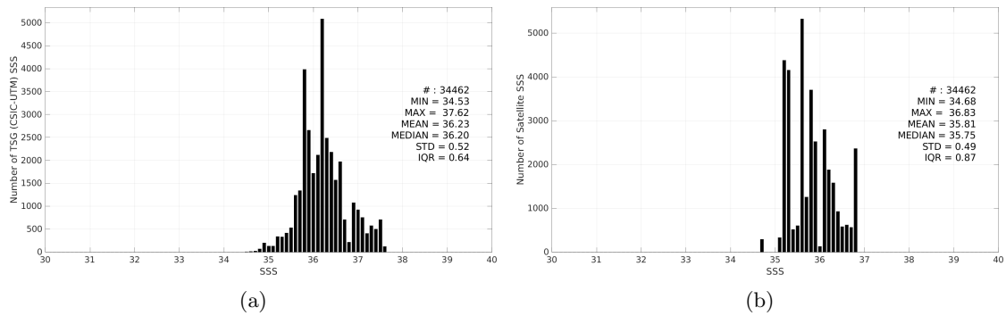
Figure 3: Histograms of SSS from TSG (CSIC-UTM) (a) and Aquarius SSS L3 CAP v5 - 7-Day running (JPL) (b) considering all match-up pairs per bins of 0.1 over the Equatorial Ocean 10N-10S Pi-MEP region and for the full satellite product period.
