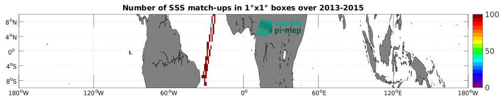
Figure 5: Number of SSS match-ups between TSG (CSIC-UTM) SSS and the Aquarius SSS L3 CAP v5 - 7-Day running (JPL) SSS product for the Equatorial Ocean 10N-10S Pi-MEP region over 1^\circ \times 1^\circ boxes and for the full satellite product period.
