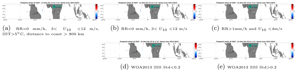
Figure 14: Temporal mean gridded over spatial boxes of size 1^\circ \times 1^\circ of \Delta SSS (Aquarius SSS L3 CAP v5 - 7-Day running (JPL) - TSG (CSIC-UTM)) for 5 different subdatasets corresponding to: RR=0 mm/h, 3 < U_{10} < 12 m/s, SST>5°C, distance to coast > 800 km (a), RR=0 mm/h, 3 < U_{10} < 12 m/s (b), RR>1mm/h and U_{10} < 4 m/s (c), WOA2013 SSS Std<0.2 (d), WOA2013 SSS Std>0.2 (e).
