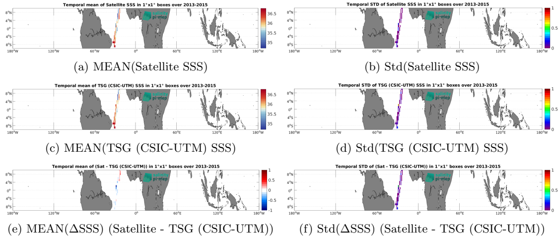
Figure 7: Temporal mean (left) and Std (right) of SSS from Aquarius SSS L3 CAP v5 - 7-Day running (JPL) (top), TSG (CSIC-UTM) (middle), and of \Delta SSS (Satellite - TSG (CSIC-UTM)). Only match-up pairs are used to generate these maps.
