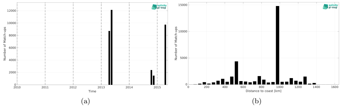
Figure 2: Number of match-ups between TSG (CSIC-UTM) and Aquarius SSS L3 CAP v5 - 7-Day running (JPL) SSS as a function of time (a) and as function of the distance to coast (b) over the Equatorial Ocean 10N-10S Pi-MEP region and for the full satellite product period.
