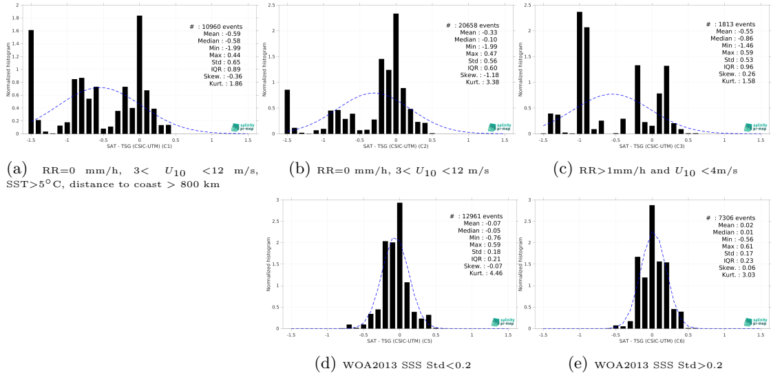
Figure 15: Normalized histogram of \Delta SSS (Aquarius SSS L3 CAP v5 - 7-Day running (JPL) - TSG (CSIC-UTM)) for 5 different subdatasets corresponding to: RR=0 mm/h, 3 < U_{10} < 12 m/s, SST>5°C, distance to coast > 800 km (a), RR=0 mm/h, 3 < U_{10} < 12 m/s (b), RR>1mm/h and U_{10} < 4 m/s (c), WOA2013 SSS Std<0.2 (d), WOA2013 SSS Std>0.2 (e).
