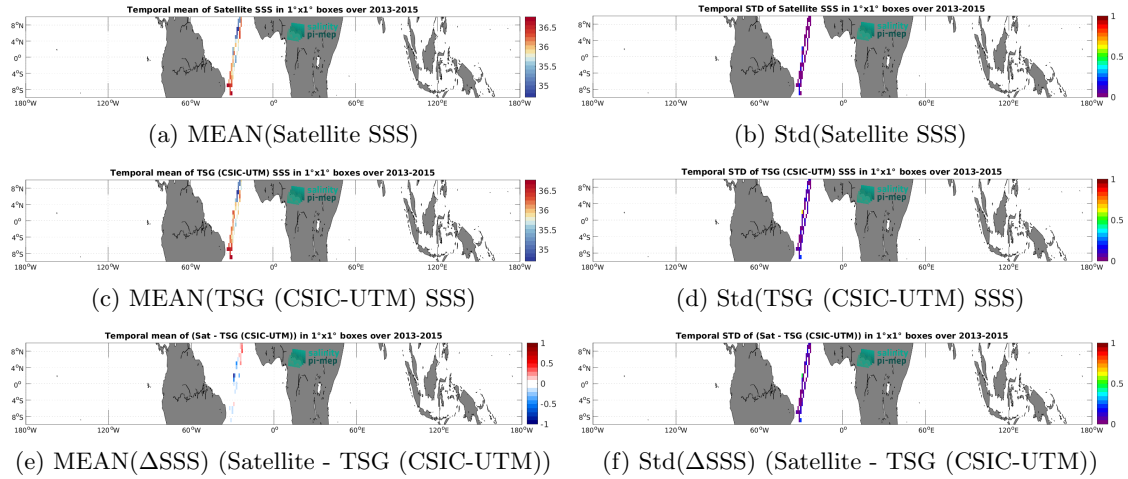
Figure 6: Temporal mean (left) and Std (right) of SSS from Aquarius SSS L3 CAP v5 - 7-Day running (JPL) (top), TSG (CSIC-UTM) (middle), and of \Delta SSS (Satellite - TSG (CSIC-UTM)). Only match-up pairs are used to generate these maps.
