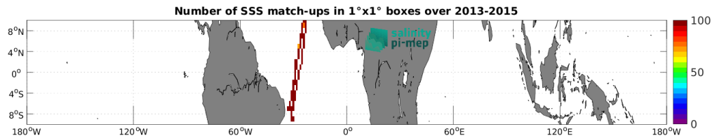
Figure 4: Number of SSS match-ups between TSG (CSIC-UTM) SSS and the Aquarius SSS L3 CAP v5 - 7-Day running (JPL) SSS product for the Equatorial Ocean 10N-10S Pi-MEP region over 1^\circ \times 1^\circ boxes and for the full satellite product period.
