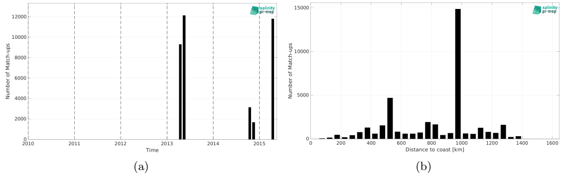
Figure 1: Number of match-ups between TSG (CSIC-UTM) and Aquarius SSS L3 CAP v5 - 7-Day running (JPL) SSS as a function of time (a) and as function of the distance to coast (b) over the Equatorial Ocean 10N-10S Pi-MEP region and for the full satellite product period.
