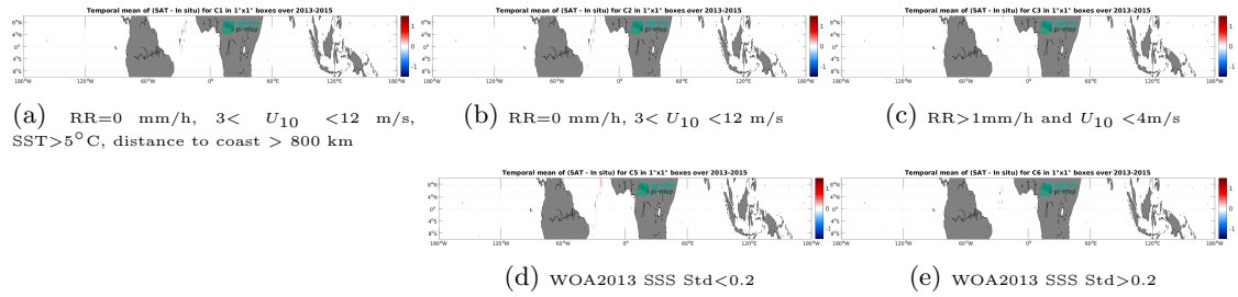
Figure 12: Temporal mean gridded over spatial boxes of size 1^\circ \times 1^\circ of \Delta\text{SSS} (Aquarius SSS L3 CAP v5 - 7-Day running (JPL) - TSG (CSIC-UTM)) for 5 different subdatasets corresponding to:RR=0 mm/h, 3 < U_{10} < 12 m/s, SST >5^\circ\text{C} , distance to coast > 800 km (a), RR=0 mm/h, 3 < U_{10} < 12 m/s (b), RR >1 mm/h and U_{10} < 4 m/s (c), WOA2013 SSS Std <0.2 (d), WOA2013 SSS Std >0.2 (e).
