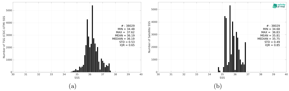
Figure 2: Histograms of SSS from TSG (CSIC-UTM) (a) and Aquarius SSS L3 CAP v5 - 7-Day running (JPL) (b) considering all match-up pairs per bins of 0.1 over the Equatorial Ocean 10N-10S Pi-MEP region and for the full satellite product period.
