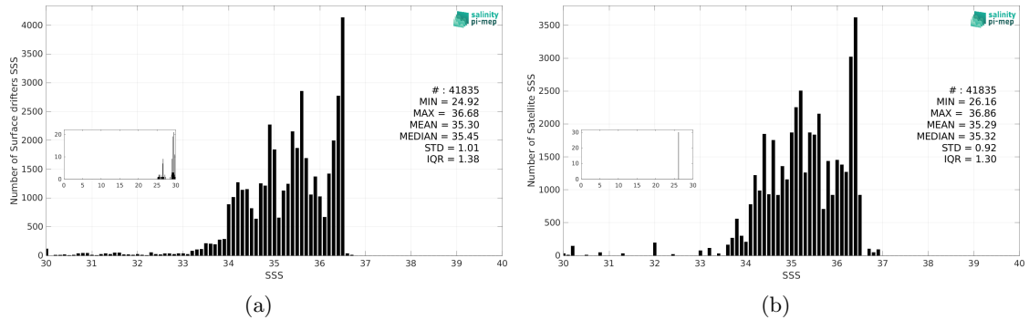
Figure 3: Histograms of SSS from Surface drifters (a) and Aquarius SSS L3 CAP v5 - 7-Day running (JPL) (b) considering all match-up pairs per bins of 0.1 over the Equatorial Ocean 10N-10S Pi-MEP region and for the full satellite product period.
