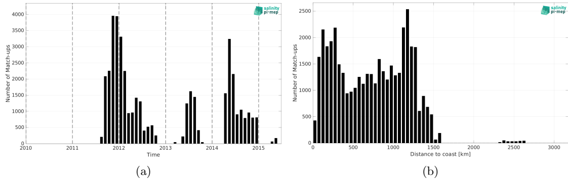
Figure 2: Number of match-ups between Surface drifters and Aquarius SSS L3 CAP v5 - 7-Day running (JPL) SSS as a function of time (a) and as function of the distance to coast (b) over the Equatorial Ocean 10N-10S Pi-MEP region and for the full satellite product period.
