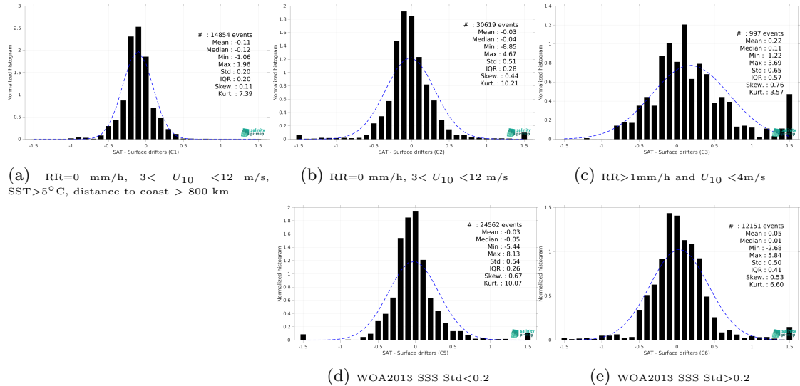
Figure 14: Normalized histogram of \Delta\text{SSS} (Aquarius SSS L3 CAP v5 - 7-Day running (JPL) - Surface drifters) for 5 different subdatasets corresponding to: RR=0 mm/h, 3 < U_{10} < 12 m/s, SST >5^\circ\text{C} , distance to coast > 800 km (a), RR=0 mm/h, 3 < U_{10} < 12 m/s (b), RR >1 mm/h and U_{10} < 4 m/s (c), WOA2013 SSS Std <0.2 (d), WOA2013 SSS Std >0.2 (e).
