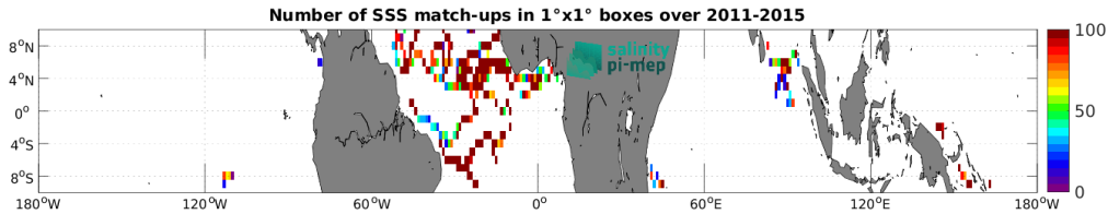
Figure 4: Number of SSS match-ups between Surface drifters SSS and the Aquarius SSS L3 CAP v5 - 7-Day running (JPL) SSS product for the Equatorial Ocean 10N-10S Pi-MEP region over 1^\circ \times 1^\circ boxes and for the full satellite product period.
