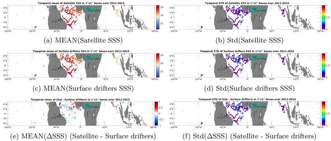
Figure 6: Temporal mean (left) and Std (right) of SSS from Aquarius SSS L3 CAP v5 - 7-Day running (JPL) (top), Surface drifters (middle), and of \Delta SSS (Satellite - Surface drifters). Only match-up pairs are used to generate these maps.
