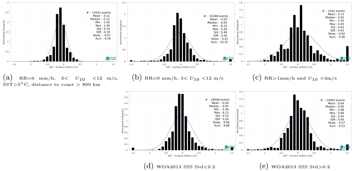
Figure 12: Normalized histogram of \Delta SSS (Aquarius SSS L3 CAP v5 - 7-Day running (JPL) - Surface drifters) for 5 different subdatasets corresponding to: RR=0 mm/h, 3 < U_{10} < 12 m/s, SST >5^\circ\text{C} , distance to coast > 800 km (a), RR=0 mm/h, 3 < U_{10} < 12 m/s (b), RR >1 mm/h and U_{10} < 4 m/s (c), WOA2013 SSS Std <0.2 (d), WOA2013 SSS Std >0.2 (e).
