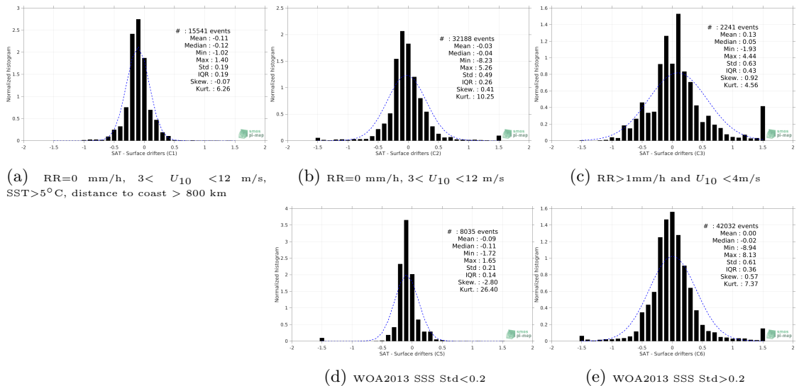
Figure 12: Normalized histogram of ΔSSS (Aquarius SSS L3 CAP v5 - 7-Day running (JPL) - Surface drifters) for 5 different subdatasets corresponding to: RR=0 mm/h, 3 < U 10 < 12 m/s, SST>5°C, distance to coast > 800 km (a), RR=0 mm/h, 3 < U 10 < 12 m/s (b), RR>1mm/h and U 10 < 4m/s (c), WOA2013 SSS Std<0.2 (d), WOA2013 SSS Std>0.2 (e).
