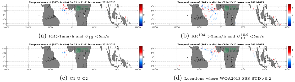
Figure 11: Temporal mean gridded over spatial boxes of size 1^\circ \times 1^\circ of \Delta SSS (Aquarius-L3-JPL-V5-7DAY-RUNNING - Surface drifters) for 4 different subdatasets corresponding to: RR > 1\text{mm/h} and U_{10} < 5\text{m/s} (a), RR^{10d} > 5\text{mm/h} and U_{10}^{10d} < 5\text{m/s} (b), C1 U C2 (c), Locations where WOA2013 SSS STD > 0.2 (d).
