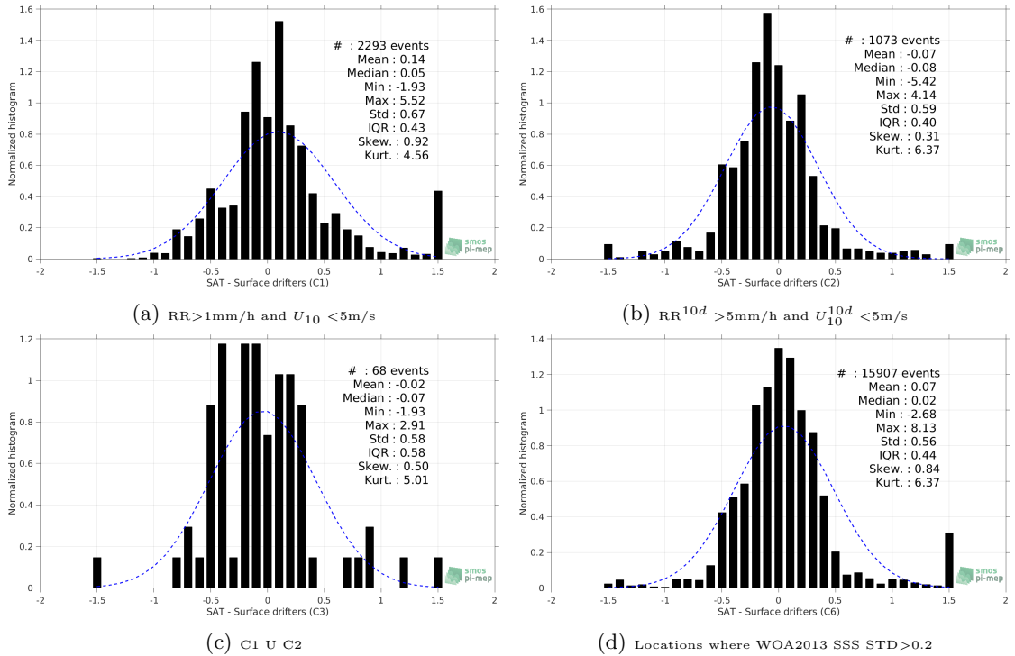
Figure 12: Normalized histogram of \Delta SSS (Aquarius-L3-JPL-V5-7DAY-RUNNING - Surface drifters) for 6 different subdatasets corresponding to: RR > 1\text{mm/h} and U_{10} < 5\text{m/s} (a), RR^{10d} > 5\text{mm/h} and U_{10}^{10d} < 5\text{m/s} (b), C1 U C2 (c), Locations where WOA2013 SSS STD > 0.2 (d).
