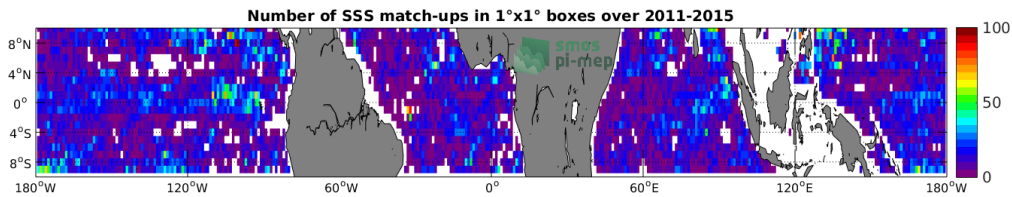
Figure 4: Number of SSS match-ups between Argo SSS and the Aquarius-L3-JPL-V5-7DAY-RUNNING SSS product for the Equatorial Ocean 10N-10S Pi-MEP region over 1^\circ \times 1^\circ boxes and for the full satellite product period.
