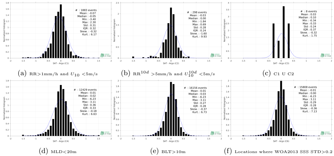
Figure 13: Normalized histogram of \Delta\text{SSS} (Aquarius-L3-JPL-V5-7DAY-RUNNING - Argo) for 6 different subdatasets corresponding to: \text{RR} > 1\text{mm/h} and U_{10} < 5\text{m/s} (a), \text{RR}^{10d} > 5\text{mm/h} and U_{10}^{10d} < 5\text{m/s} (b), C1 U C2 (c), \text{MLD} < 20\text{m} (d), \text{BLT} > 10\text{m} (e), Locations where WOA2013 SSS \text{STD} > 0.2 (f).
