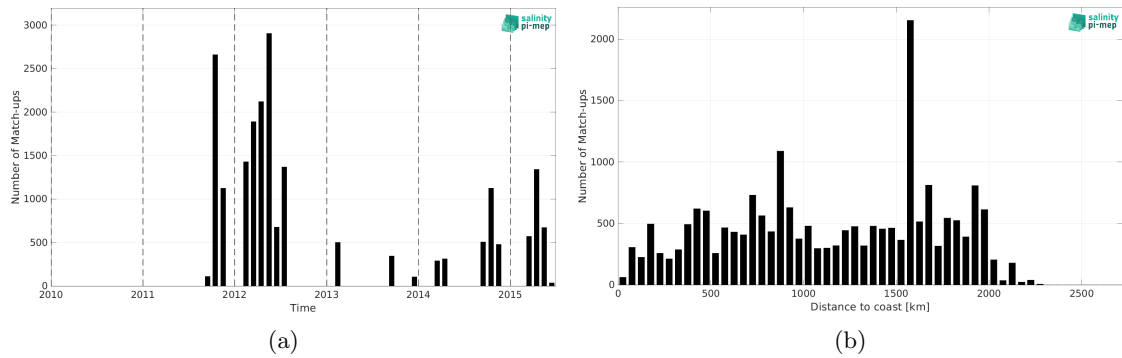
Figure 2: Number of match-ups between TSG (SAMOS) and Aquarius SSS L3 CAP v5 - Monthly (JPL) SSS as a function of time (a) and as function of the distance to coast (b) over the Equatorial Ocean 10N-10S Pi-MEP region and for the full satellite product period.
