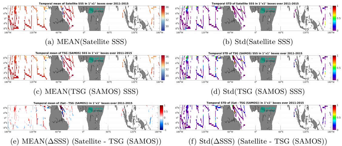
Figure 7: Temporal mean (left) and Std (right) of SSS from Aquarius SSS L3 CAP v5 - Monthly (JPL) (top), TSG (SAMOS) (middle), and of \Delta SSS (Satellite - TSG (SAMOS)). Only match-up pairs are used to generate these maps.
