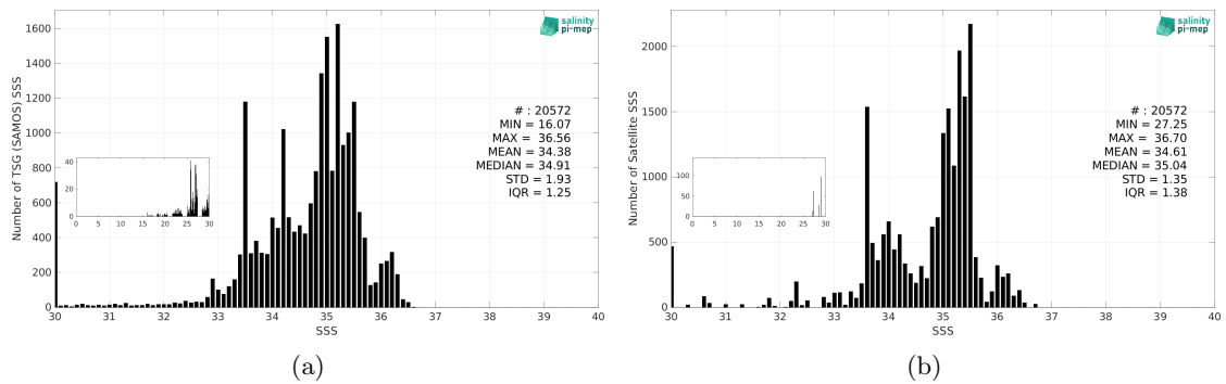
Figure 3: Histograms of SSS from TSG (SAMOS) (a) and Aquarius SSS L3 CAP v5 - Monthly (JPL) (b) considering all match-up pairs per bins of 0.1 over the Equatorial Ocean 10N-10S Pi-MEP region and for the full satellite product period.
