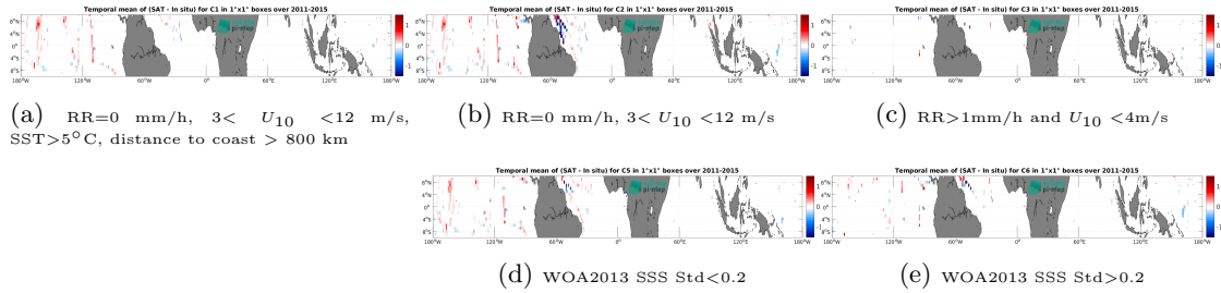
Figure 14: Temporal mean gridded over spatial boxes of size 1^\circ \times 1^\circ of \Delta SSS (Aquarius SSS L3 CAP v5 - Monthly (JPL) - TSG (SAMOS)) for 5 different subdatasets corresponding to: RR=0 mm/h, 3 < U_{10} < 12 m/s, SST>5°C, distance to coast > 800 km (a), RR=0 mm/h, 3 < U_{10} < 12 m/s (b), RR>1mm/h and U_{10} < 4 m/s (c), WOA2013 SSS Std<0.2 (d), WOA2013 SSS Std>0.2 (e).
