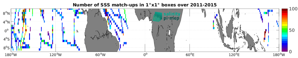
Figure 5: Number of SSS match-ups between TSG (SAMOS) SSS and the Aquarius SSS L3 CAP v5 - Monthly (JPL) SSS product for the Equatorial Ocean 10N-10S Pi-MEP region over 1^\circ \times 1^\circ boxes and for the full satellite product period.
