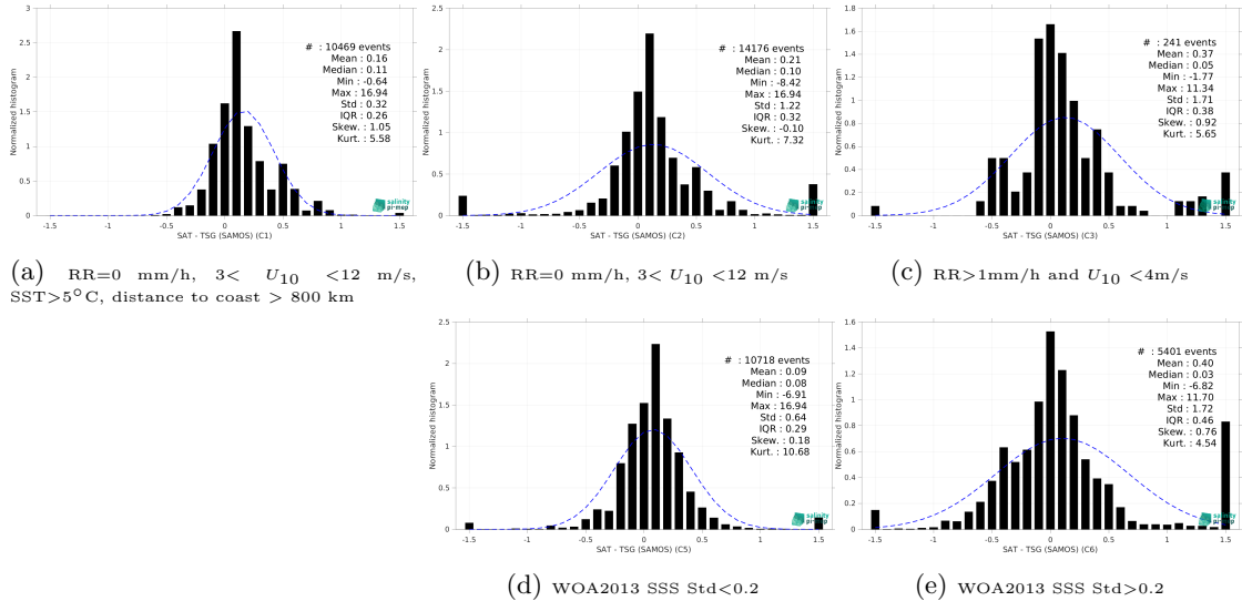
Figure 15: Normalized histogram of \Delta SSS (Aquarius SSS L3 CAP v5 - Monthly (JPL) - TSG (SAMOS)) for 5 different subdatasets corresponding to: RR=0 mm/h, 3 < U_{10} < 12 m/s, SST>5°C, distance to coast > 800 km (a), RR=0 mm/h, 3 < U_{10} < 12 m/s (b), RR>1mm/h and U_{10} < 4 m/s (c), WOA2013 SSS Std<0.2 (d), WOA2013 SSS Std>0.2 (e).
