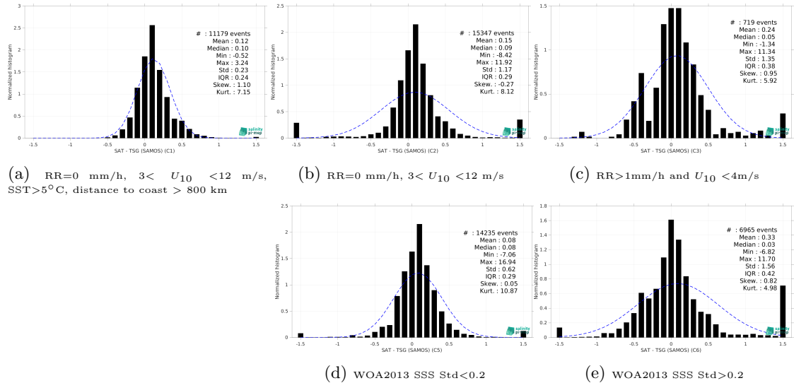
Figure 13: Normalized histogram of \Delta\text{SSS} (Aquarius SSS L3 CAP v5 - Monthly (JPL) - TSG (SAMOS)) for 5 different subdatasets corresponding to: \text{RR}=0 mm/h, 3 < U_{10} < 12 m/s, \text{SST} > 5^\circ\text{C} , distance to coast > 800 km (a), \text{RR}=0 mm/h, 3 < U_{10} < 12 m/s (b), \text{RR} > 1\text{mm/h} and U_{10} < 4\text{m/s} (c), WOA2013 SSS Std < 0.2 (d), WOA2013 SSS Std > 0.2 (e).
