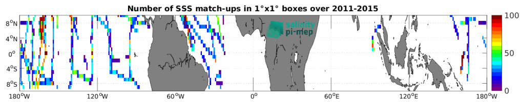
Figure 4: Number of SSS match-ups between TSG (SAMOS) SSS and the Aquarius SSS L3 CAP v5 - Monthly (JPL) SSS product for the Equatorial Ocean 10N-10S Pi-MEP region over 1^\circ \times 1^\circ boxes and for the full satellite product period.
