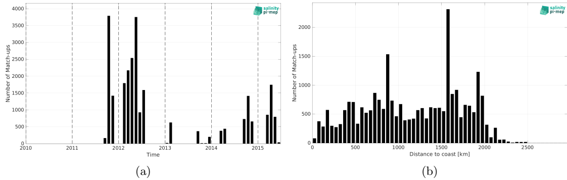
Figure 1: Number of match-ups between TSG (SAMOS) and Aquarius SSS L3 CAP v5 - Monthly (JPL) SSS as a function of time (a) and as function of the distance to coast (b) over the Equatorial Ocean 10N-10S Pi-MEP region and for the full satellite product period.
