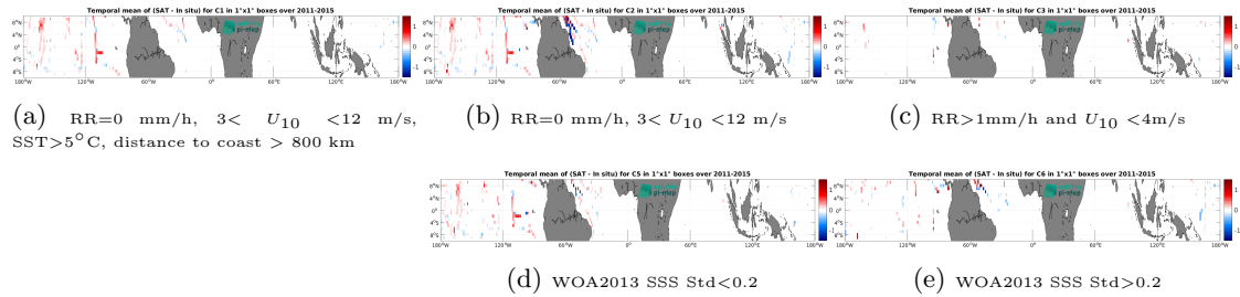
Figure 12: Temporal mean gridded over spatial boxes of size 1^\circ \times 1^\circ of \Delta\text{SSS} (Aquarius SSS L3 CAP v5 - Monthly (JPL) - TSG (SAMOS)) for 5 different subdatasets corresponding to: \text{RR}=0 mm/h, 3 < U_{10} < 12 m/s, \text{SST} > 5^\circ\text{C} , distance to coast > 800 km (a), \text{RR}=0 mm/h, 3 < U_{10} < 12 m/s (b), \text{RR} > 1\text{mm/h} and U_{10} < 4\text{m/s} (c), WOA2013 SSS Std < 0.2 (d), WOA2013 SSS Std > 0.2 (e).
