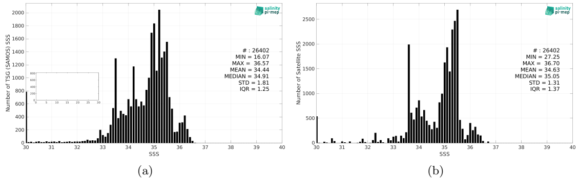
Figure 2: Histograms of SSS from TSG (SAMOS) (a) and Aquarius SSS L3 CAP v5 - Monthly (JPL) (b) considering all match-up pairs per bins of 0.1 over the Equatorial Ocean 10N-10S Pi-MEP region and for the full satellite product period.
