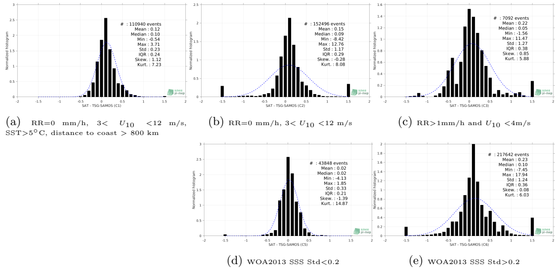
Figure 13: Normalized histogram of \Delta SSS (Aquarius-L3-JPL-V5-MONTHLY - TSG-SAMOS) for 5 different subdatasets corresponding to: RR=0 mm/h, 3 < U_{10} < 12 m/s, SST >5^\circ\text{C} , distance to coast > 800 km (a), RR=0 mm/h, 3 < U_{10} < 12 m/s (b), RR >1 mm/h and U_{10} < 4 m/s (c), WOA2013 SSS Std <0.2 (d), WOA2013 SSS Std >0.2 (e).
