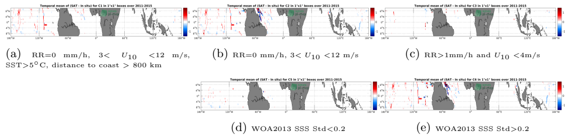
Figure 12: Temporal mean gridded over spatial boxes of size 1^\circ \times 1^\circ of \Delta SSS (Aquarius-L3-JPL-V5-MONTHLY - TSG-SAMOS) for 5 different subdatasets corresponding to:RR=0 mm/h, 3 < U_{10} < 12 m/s, SST >5^\circ\text{C} , distance to coast > 800 km (a), RR=0 mm/h, 3 < U_{10} < 12 m/s (b), RR >1 mm/h and U_{10} < 4 m/s (c), WOA2013 SSS Std <0.2 (d), WOA2013 SSS Std >0.2 (e).
