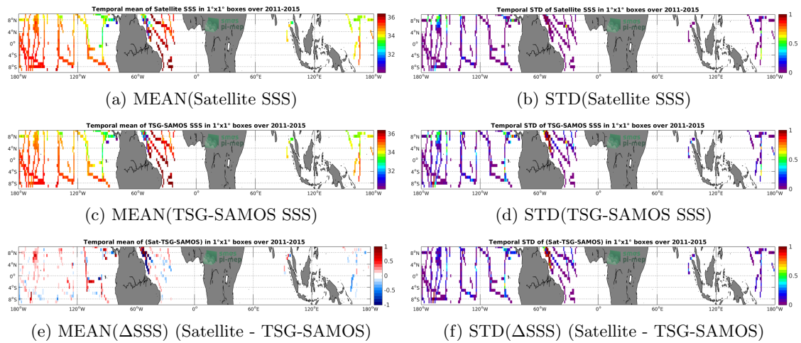
Figure 6: Temporal mean (left) and STD (right) of SSS from Aquarius-L3-JPL-V5-MONTHLY (top), TSG-SAMOS (middle), and of \Delta SSS (Satellite - TSG-SAMOS). Only match-up pairs are used to generate these maps.
