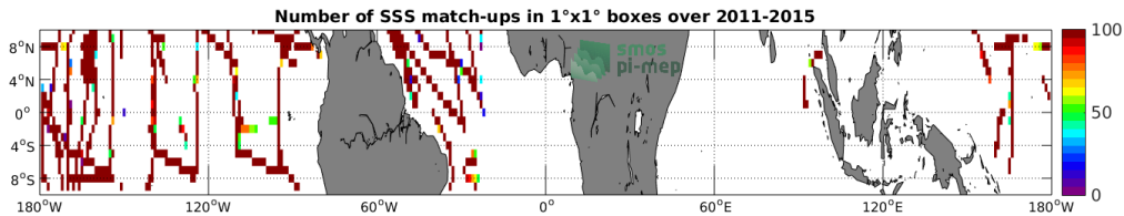
Figure 4: Number of SSS match-ups between TSG-SAMOS SSS and the Aquarius-L3-JPL-V5-MONTHLY SSS product for the Equatorial Ocean 10N-10S Pi-MEP region over 1^\circ \times 1^\circ boxes and for the full satellite product period.
