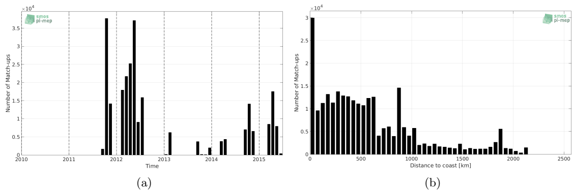
Figure 1: Number of match-ups between TSG-SAMOS and Aquarius-L3-JPL-V5-MONTHLY SSS as a function of time (a) and as function of the distance to coast (b) over the Equatorial Ocean 10N-10S Pi-MEP region and for the full satellite product period.
