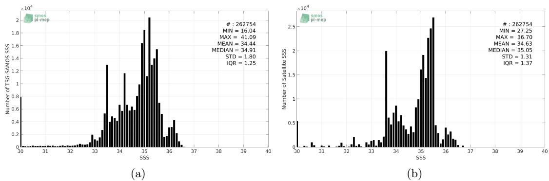
Figure 2: Histograms of SSS from TSG-SAMOS (a) and Aquarius-L3-JPL-V5-MONTHLY (b) considering all match-up pairs per bins of 0.1 over the Equatorial Ocean 10N-10S Pi-MEP region and for the full satellite product period.
