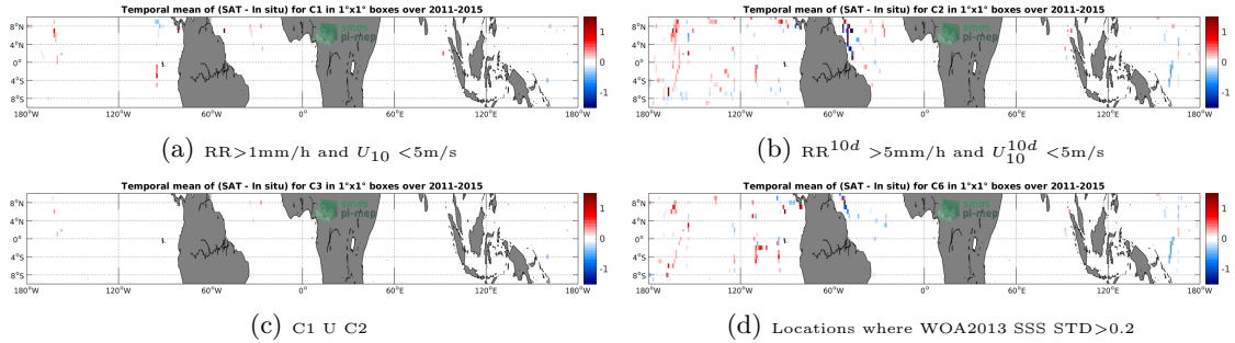
Figure 12: Temporal mean gridded over spatial boxes of size 1^\circ \times 1^\circ of \Delta SSS (Aquarius-L3-JPL-V5-MONTHLY - TSG-SAMOS) for 4 different subdatasets corresponding to: RR > 1\text{mm/h} and U_{10} < 5\text{m/s} (a), RR^{10d} > 5\text{mm/h} and U_{10}^{10d} < 5\text{m/s} (b), C1 U C2 (c), Locations where WOA2013 SSS STD > 0.2 (d).
