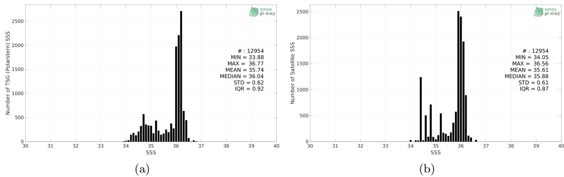
Figure 2: Histograms of SSS from TSG (Polarstern) (a) and Aquarius SSS L3 CAP v5 - Monthly (JPL) (b) considering all match-up pairs per bins of 0.1 over the Equatorial Ocean 10N-10S Pi-MEP region and for the full satellite product period.
