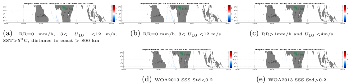
Figure 12: Temporal mean gridded over spatial boxes of size 1^\circ \times 1^\circ of \Delta SSS (Aquarius SSS L3 CAP v5 - Monthly (JPL) - TSG (Polarstern)) for 5 different subdatasets corresponding to: RR=0 mm/h, 3 < U_{10} < 12 m/s, SST >5^\circ C, distance to coast > 800 km (a), RR=0 mm/h, 3 < U_{10} < 12 m/s (b), RR >1 mm/h and U_{10} < 4 m/s (c), WOA2013 SSS Std <0.2 (d), WOA2013 SSS Std >0.2 (e).
