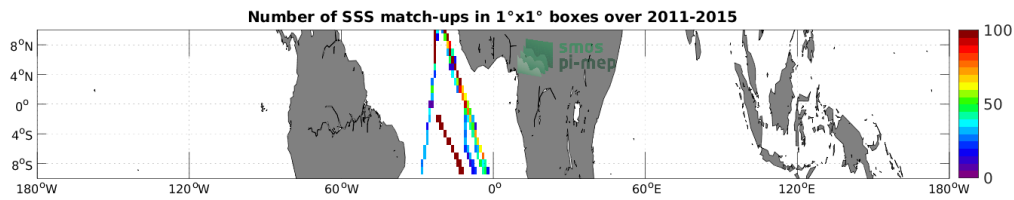
Figure 4: Number of SSS match-ups between TSG (Polarstern) SSS and the Aquarius SSS L3 CAP v5 - Monthly (JPL) SSS product for the Equatorial Ocean 10N-10S Pi-MEP region over 1^\circ \times 1^\circ boxes and for the full satellite product period.
