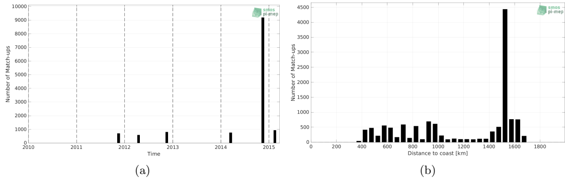
Figure 1: Number of match-ups between TSG (Polarstern) and Aquarius SSS L3 CAP v5 - Monthly (JPL) SSS as a function of time (a) and as function of the distance to coast (b) over the Equatorial Ocean 10N-10S Pi-MEP region and for the full satellite product period.
