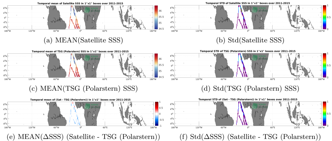
Figure 6: Temporal mean (left) and Std (right) of SSS from Aquarius SSS L3 CAP v5 - Monthly (JPL) (top), TSG (Polarstern) (middle), and of \Delta SSS (Satellite - TSG (Polarstern)). Only match-up pairs are used to generate these maps.
