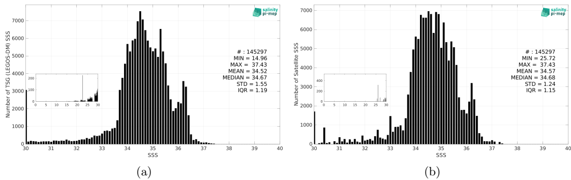
Figure 3: Histograms of SSS from TSG (LEGOS-DM) (a) and Aquarius SSS L3 CAP v5 - Monthly (JPL) (b) considering all match-up pairs per bins of 0.1 over the Equatorial Ocean 10N-10S Pi-MEP region and for the full satellite product period.
