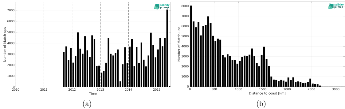
Figure 2: Number of match-ups between TSG (LEGOS-DM) and Aquarius SSS L3 CAP v5 - Monthly (JPL) SSS as a function of time (a) and as function of the distance to coast (b) over the Equatorial Ocean 10N-10S Pi-MEP region and for the full satellite product period.
