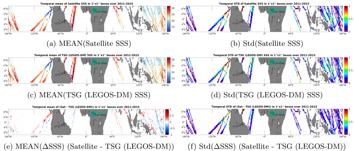
Figure 7: Temporal mean (left) and Std (right) of SSS from Aquarius SSS L3 CAP v5 - Monthly (JPL) (top), TSG (LEGOS-DM) (middle), and of \Delta SSS (Satellite - TSG (LEGOS-DM)). Only match-up pairs are used to generate these maps.
