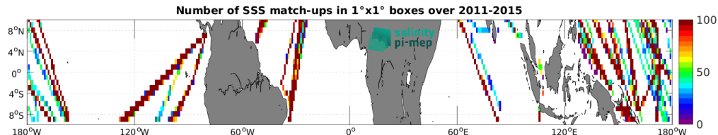
Figure 5: Number of SSS match-ups between TSG (LEGOS-DM) SSS and the Aquarius SSS L3 CAP v5 - Monthly (JPL) SSS product for the Equatorial Ocean 10N-10S Pi-MEP region over 1^\circ \times 1^\circ boxes and for the full satellite product period.
