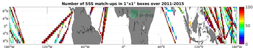
Figure 4: Number of SSS match-ups between TSG (LEGOS-DM) SSS and the Aquarius SSS L3 CAP v5 - Monthly (JPL) SSS product for the Equatorial Ocean 10N-10S Pi-MEP region over 1^\circ \times 1^\circ boxes and for the full satellite product period.
