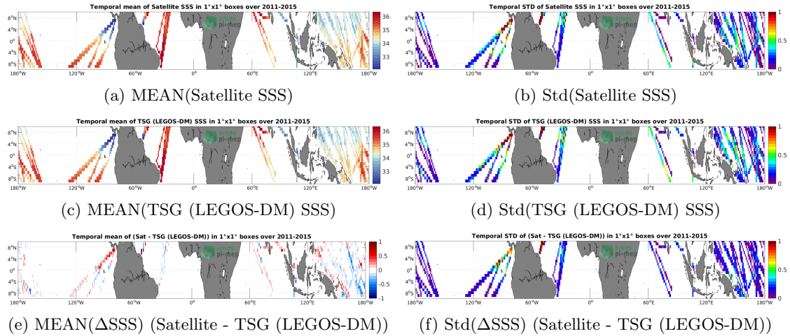
Figure 6: Temporal mean (left) and Std (right) of SSS from Aquarius SSS L3 CAP v5 - Monthly (JPL) (top), TSG (LEGOS-DM) (middle), and of \Delta SSS (Satellite - TSG (LEGOS-DM)). Only match-up pairs are used to generate these maps.
