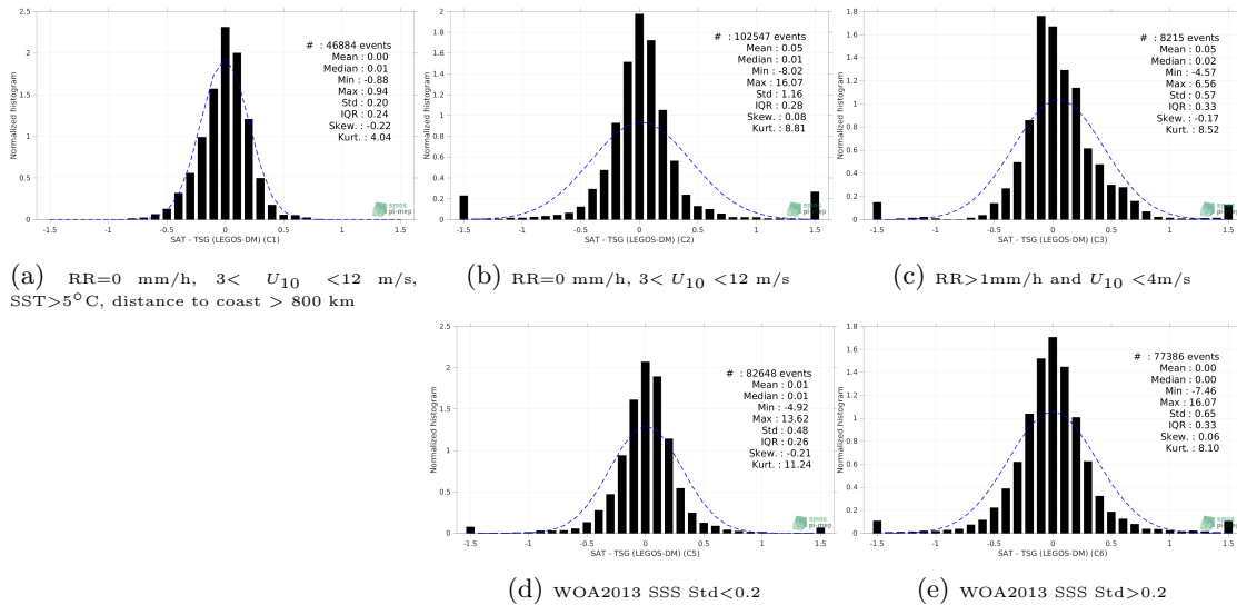
Figure 13: Normalized histogram of \Delta SSS (Aquarius SSS L3 CAP v5 - Monthly (JPL) - TSG (LEGOS-DM)) for 5 different subdatasets corresponding to: RR=0 mm/h, 3 < U_{10} < 12 m/s, SST >5^\circ\text{C} , distance to coast > 800 km (a), RR=0 mm/h, 3 < U_{10} < 12 m/s (b), RR >1 mm/h and U_{10} < 4 m/s (c), WOA2013 SSS Std <0.2 (d), WOA2013 SSS Std >0.2 (e).
