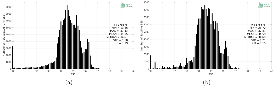
Figure 2: Histograms of SSS from TSG (LEGOS-DM) (a) and Aquarius SSS L3 CAP v5 - Monthly (JPL) (b) considering all match-up pairs per bins of 0.1 over the Equatorial Ocean 10N-10S Pi-MEP region and for the full satellite product period.
