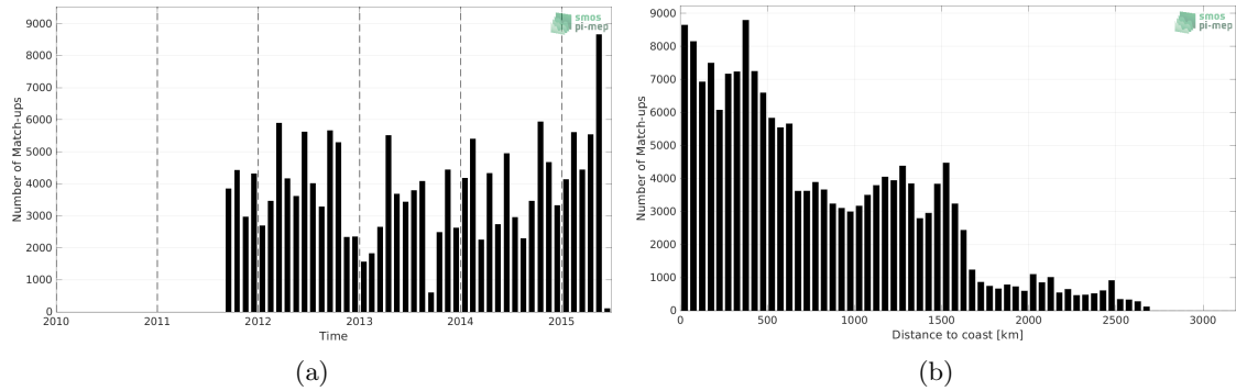
Figure 1: Number of match-ups between TSG (LEGOS-DM) and Aquarius SSS L3 CAP v5 - Monthly (JPL) SSS as a function of time (a) and as function of the distance to coast (b) over the Equatorial Ocean 10N-10S Pi-MEP region and for the full satellite product period.
