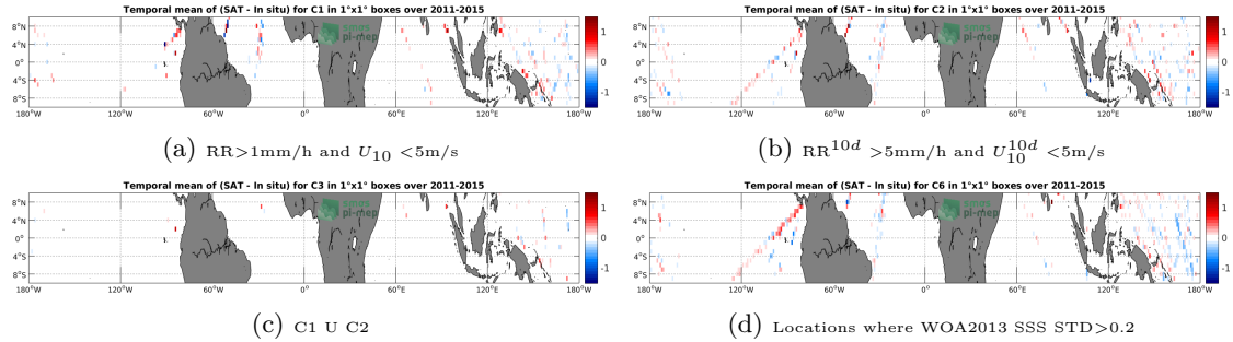
Figure 12: Temporal mean gridded over spatial boxes of size 1^\circ \times 1^\circ of \Delta SSS (Aquarius-L3-JPL-V5-MONTHLY - TSG-LEGOS-DM) for 4 different subdatasets corresponding to: RR > 1\text{mm/h} and U_{10} < 5\text{m/s} (a), RR^{10d} > 5\text{mm/h} and U_{10}^{10d} < 5\text{m/s} (b), C1 U C2 (c), Locations where WOA2013 SSS STD > 0.2 (d).
