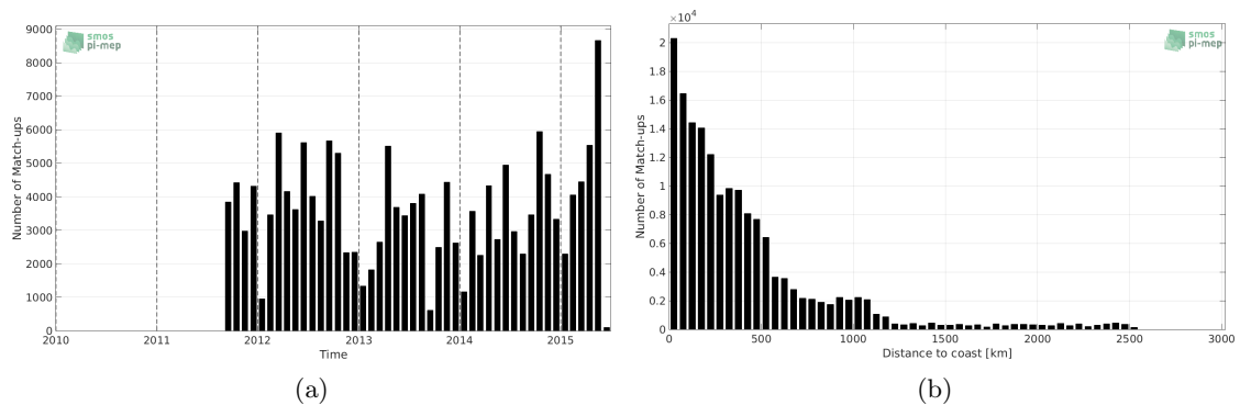
Figure 1: Number of match-ups between TSG-LEGOS-DM and Aquarius-L3-JPL-V5-MONTHLY SSS as a function of time (a) and as function of the distance to coast (b) over the Equatorial Ocean 10N-10S Pi-MEP region and for the full satellite product period.
