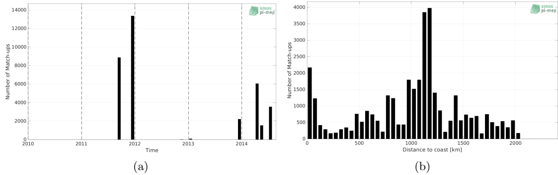
Figure 1: Number of match-ups between TSG (GOSUD-Sailing-ship) and Aquarius SSS L3 CAP v5 - Monthly (JPL) SSS as a function of time (a) and as function of the distance to coast (b) over the Equatorial Ocean 10N-10S Pi-MEP region and for the full satellite product period.
