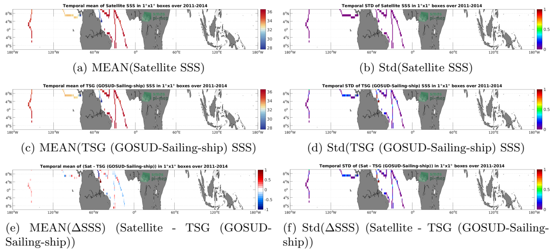
Figure 6: Temporal mean (left) and Std (right) of SSS from Aquarius SSS L3 CAP v5 - Monthly (JPL) (top), TSG (GOSUD-Sailing-ship) (middle), and of \Delta SSS (Satellite - TSG (GOSUD-Sailing-ship)). Only match-up pairs are used to generate these maps.
