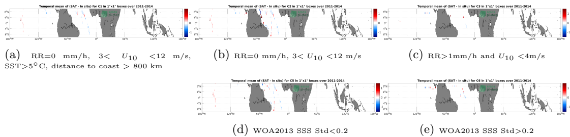
Figure 12: Temporal mean gridded over spatial boxes of size 1^\circ \times 1^\circ of \Delta SSS (Aquarius SSS L3 CAP v5 - Monthly (JPL) - TSG (GOSUD-Sailing-ship)) for 5 different subdatasets corresponding to: RR=0 mm/h, 3 < U_{10} < 12 m/s, SST>5°C, distance to coast > 800 km (a), RR=0 mm/h, 3 < U_{10} < 12 m/s (b), RR>1mm/h and U_{10} < 4 m/s (c), WOA2013 SSS Std<0.2 (d), WOA2013 SSS Std>0.2 (e).
