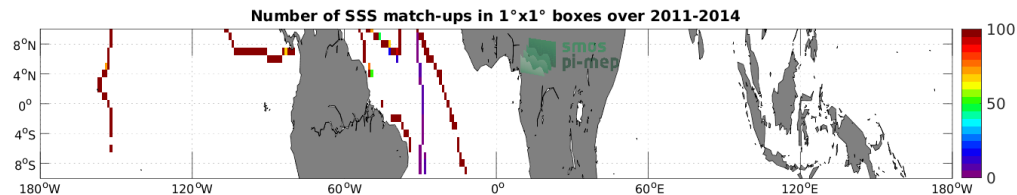
Figure 4: Number of SSS match-ups between TSG (GOSUD-Sailing-ship) SSS and the Aquarius SSS L3 CAP v5 - Monthly (JPL) SSS product for the Equatorial Ocean 10N-10S Pi-MEP region over 1^\circ \times 1^\circ boxes and for the full satellite product period.
