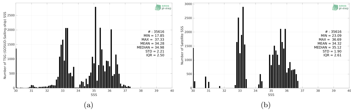
Figure 2: Histograms of SSS from TSG (GOSUD-Sailing-ship) (a) and Aquarius SSS L3 CAP v5 - Monthly (JPL) (b) considering all match-up pairs per bins of 0.1 over the Equatorial Ocean 10N-10S Pi-MEP region and for the full satellite product period.
