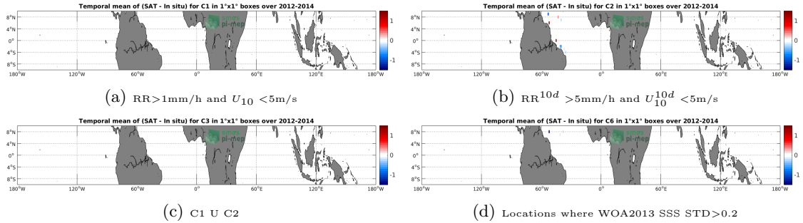
Figure 12: Temporal mean gridded over spatial boxes of size 1^\circ \times 1^\circ of \Delta SSS (Aquarius-L3-JPL-V5-MONTHLY - TSG-GOSUD-Sailing-ship) for 4 different subdatasets corresponding to: RR > 1\text{mm/h} and U_{10} < 5\text{m/s} (a), RR^{10d} > 5\text{mm/h} and U_{10}^{10d} < 5\text{m/s} (b), C1 U C2 (c), Locations where WOA2013 SSS STD > 0.2 (d).
