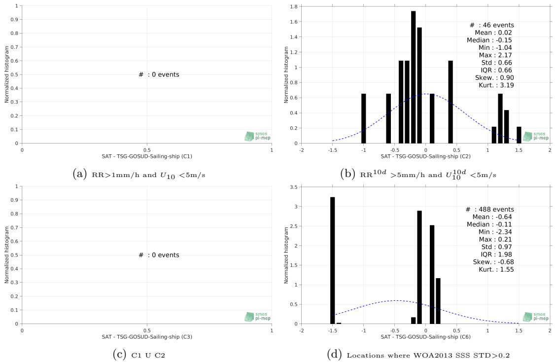
Figure 13: Normalized histogram of \Delta SSS (Aquarius-L3-JPL-V5-MONTHLY - TSG-GOSUD-Sailing-ship) for 6 different subdatasets corresponding to: RR > 1\text{mm/h} and U_{10} < 5\text{m/s} (a), RR^{10d} > 5\text{mm/h} and U_{10}^{10d} < 5\text{m/s} (b), C1 U C2 (c), Locations where WOA2013 SSS STD > 0.2 (d).
