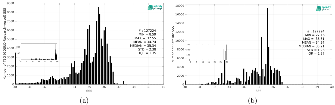
Figure 3: Histograms of SSS from TSG (GOSUD-Research-vessel) (a) and Aquarius SSS L3 CAP v5 - Monthly (JPL) (b) considering all match-up pairs per bins of 0.1 over the Equatorial Ocean 10N-10S Pi-MEP region and for the full satellite product period.
