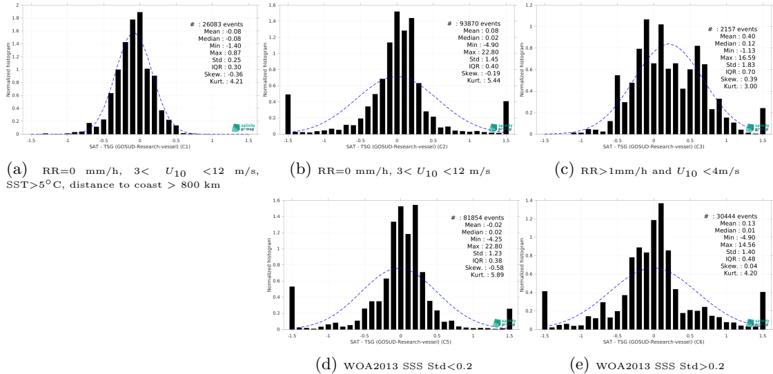
Figure 15: Normalized histogram of \Delta\text{SSS} (Aquarius SSS L3 CAP v5 - Monthly (JPL) - TSG (GOSUD-Research-vessel)) for 5 different subdatasets corresponding to: RR=0 mm/h, 3 < U_{10} < 12 m/s, SST>5°C, distance to coast > 800 km (a), RR=0 mm/h, 3 < U_{10} < 12 m/s (b), RR>1mm/h and U_{10} < 4 m/s (c), WOA2013 SSS Std<0.2 (d), WOA2013 SSS Std>0.2 (e).
