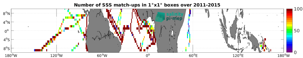
Figure 5: Number of SSS match-ups between TSG (GOSUD-Research-vessel) SSS and the Aquarius SSS L3 CAP v5 - Monthly (JPL) SSS product for the Equatorial Ocean 10N-10S Pi-MEP region over 1^\circ \times 1^\circ boxes and for the full satellite product period.
