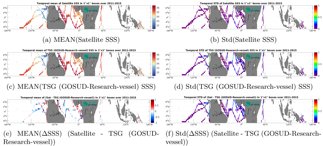
Figure 7: Temporal mean (left) and Std (right) of SSS from Aquarius SSS L3 CAP v5 - Monthly (JPL) (top), TSG (GOSUD-Research-vessel) (middle), and of \Delta SSS (Satellite - TSG (GOSUD-Research-vessel)). Only match-up pairs are used to generate these maps.
