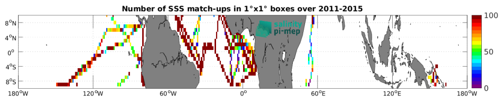
Figure 4: Number of SSS match-ups between TSG (GOSUD-Research-vessel) SSS and the Aquarius SSS L3 CAP v5 - Monthly (JPL) SSS product for the Equatorial Ocean 10N-10S Pi-MEP region over 1°x1° boxes and for the full satellite product period.
