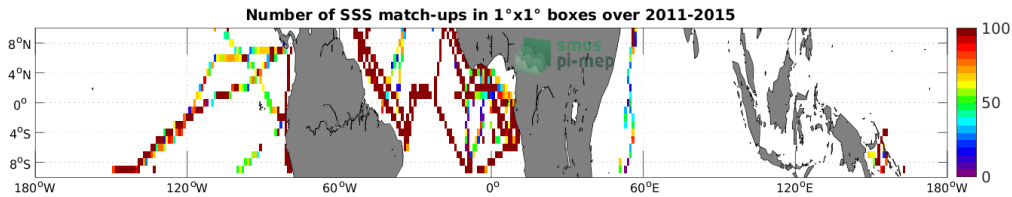
Figure 4: Number of SSS match-ups between TSG (GOSUD-Research-vessel) SSS and the Aquarius SSS L3 CAP v5 - Monthly (JPL) SSS product for the Equatorial Ocean 10N-10S Pi-MEP region over 1^\circ \times 1^\circ boxes and for the full satellite product period.
