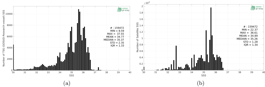
Figure 2: Histograms of SSS from TSG (GOSUD-Research-vessel) (a) and Aquarius SSS L3 CAP v5 - Monthly (JPL) (b) considering all match-up pairs per bins of 0.1 over the Equatorial Ocean 10N-10S Pi-MEP region and for the full satellite product period.
