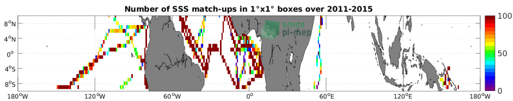
Figure 4: Number of SSS match-ups between TSG (GOSUD-Research-vessel) SSS and the Aquarius SSS L3 CAP v5 - Monthly (JPL) SSS product for the Equatorial Ocean 10N-10S Pi-MEP region over 1^\circ \times 1^\circ boxes and for the full satellite product period.
