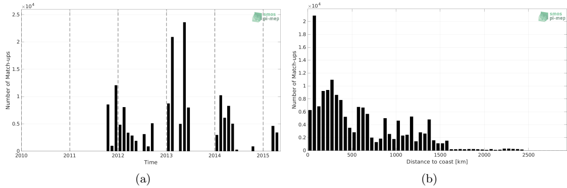
Figure 1: Number of match-ups between TSG (GOSUD-Research-vessel) and Aquarius SSS L3 CAP v5 - Monthly (JPL) SSS as a function of time (a) and as function of the distance to coast (b) over the Equatorial Ocean 10N-10S Pi-MEP region and for the full satellite product period.
