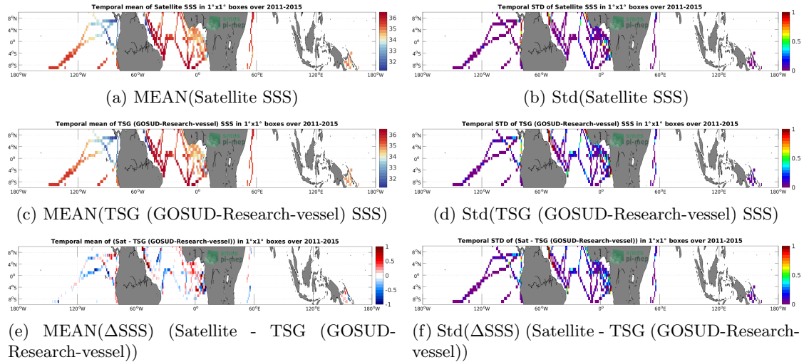
Figure 6: Temporal mean (left) and Std (right) of SSS from Aquarius SSS L3 CAP v5 - Monthly (JPL) (top), TSG (GOSUD-Research-vessel) (middle), and of \Delta SSS (Satellite - TSG (GOSUD-Research-vessel)). Only match-up pairs are used to generate these maps.
