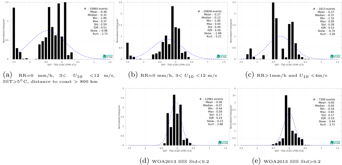
Figure 15: Normalized histogram of \Delta SSS (Aquarius SSS L3 CAP v5 - Monthly (JPL) - TSG (CSIC-UTM)) for 5 different subdatasets corresponding to: RR=0 mm/h, 3 < U_{10} < 12 m/s, SST>5°C, distance to coast > 800 km (a), RR=0 mm/h, 3 < U_{10} < 12 m/s (b), RR>1mm/h and U_{10} < 4 m/s (c), WOA2013 SSS Std<0.2 (d), WOA2013 SSS Std>0.2 (e).
