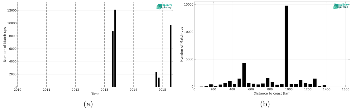
Figure 2: Number of match-ups between TSG (CSIC-UTM) and Aquarius SSS L3 CAP v5 - Monthly (JPL) SSS as a function of time (a) and as function of the distance to coast (b) over the Equatorial Ocean 10N-10S Pi-MEP region and for the full satellite product period.
