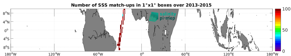
Figure 5: Number of SSS match-ups between TSG (CSIC-UTM) SSS and the Aquarius SSS L3 CAP v5 - Monthly (JPL) SSS product for the Equatorial Ocean 10N-10S Pi-MEP region over 1^\circ \times 1^\circ boxes and for the full satellite product period.
