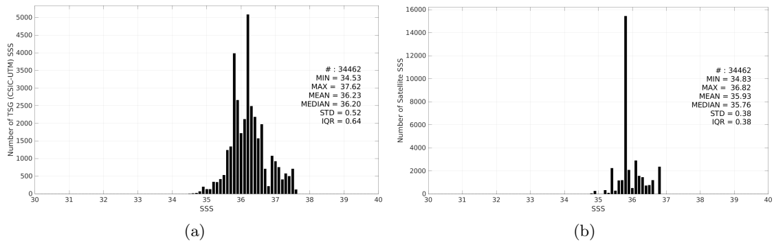
Figure 3: Histograms of SSS from TSG (CSIC-UTM) (a) and Aquarius SSS L3 CAP v5 - Monthly (JPL) (b) considering all match-up pairs per bins of 0.1 over the Equatorial Ocean 10N-10S Pi-MEP region and for the full satellite product period.
