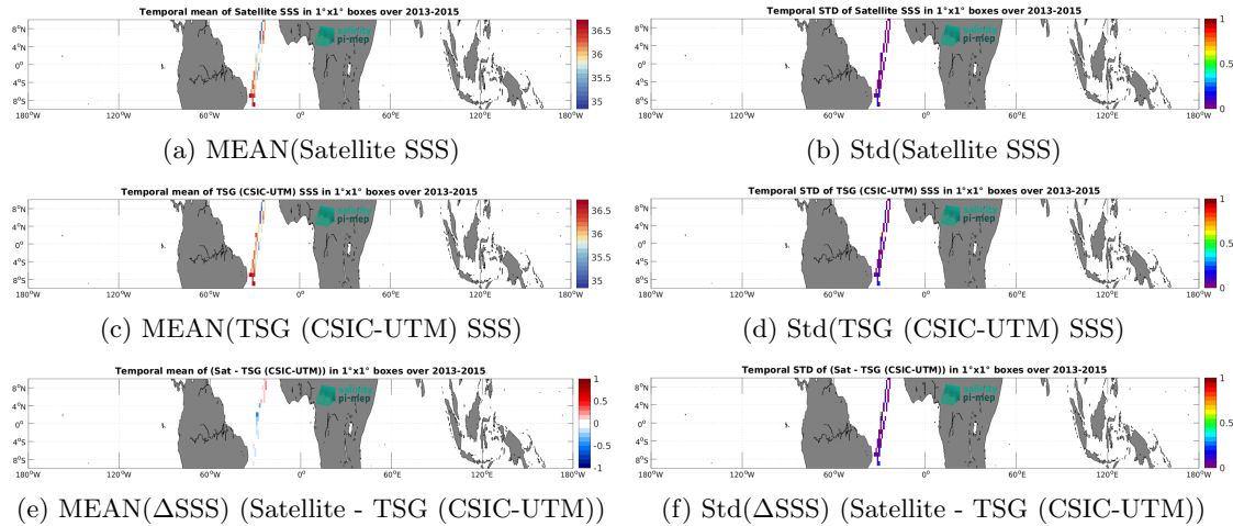
Figure 7: Temporal mean (left) and Std (right) of SSS from Aquarius SSS L3 CAP v5 - Monthly (JPL) (top), TSG (CSIC-UTM) (middle), and of \Delta SSS (Satellite - TSG (CSIC-UTM)). Only match-up pairs are used to generate these maps.
