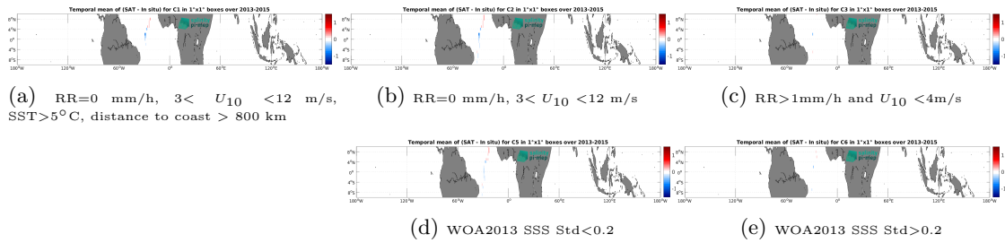
Figure 14: Temporal mean gridded over spatial boxes of size 1^\circ \times 1^\circ of \Delta SSS (Aquarius SSS L3 CAP v5 - Monthly (JPL) - TSG (CSIC-UTM)) for 5 different subdatasets corresponding to: RR=0 mm/h, 3 < U_{10} < 12 m/s, SST>5°C, distance to coast > 800 km (a), RR=0 mm/h, 3 < U_{10} < 12 m/s (b), RR>1mm/h and U_{10} < 4 m/s (c), WOA2013 SSS Std<0.2 (d), WOA2013 SSS Std>0.2 (e).
