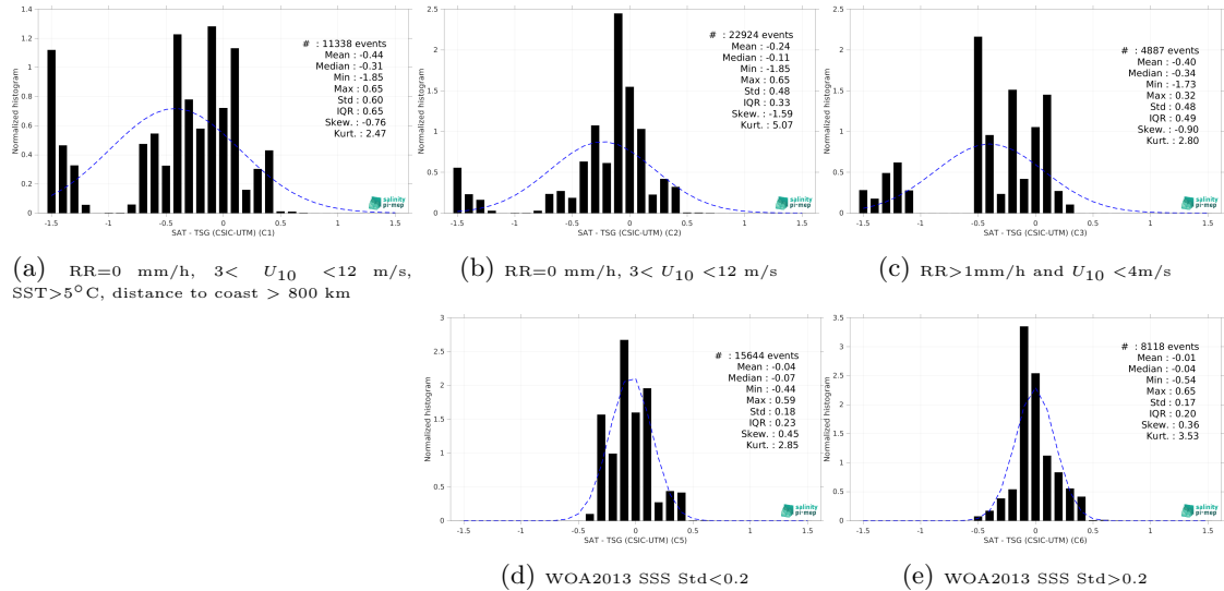
Figure 13: Normalized histogram of \Delta SSS (Aquarius SSS L3 CAP v5 - Monthly (JPL) - TSG (CSIC-UTM)) for 5 different subdatasets corresponding to: RR=0 mm/h, 3 < U_{10} < 12 m/s, SST >5^\circ C, distance to coast > 800 km (a), RR=0 mm/h, 3 < U_{10} < 12 m/s (b), RR >1 mm/h and U_{10} < 4 m/s (c), WOA2013 SSS Std <0.2 (d), WOA2013 SSS Std >0.2 (e).
