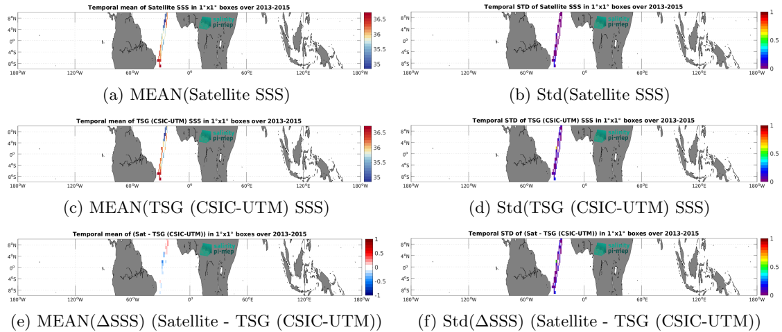
Figure 6: Temporal mean (left) and Std (right) of SSS from Aquarius SSS L3 CAP v5 - Monthly (JPL) (top), TSG (CSIC-UTM) (middle), and of \Delta SSS (Satellite - TSG (CSIC-UTM)). Only match-up pairs are used to generate these maps.
