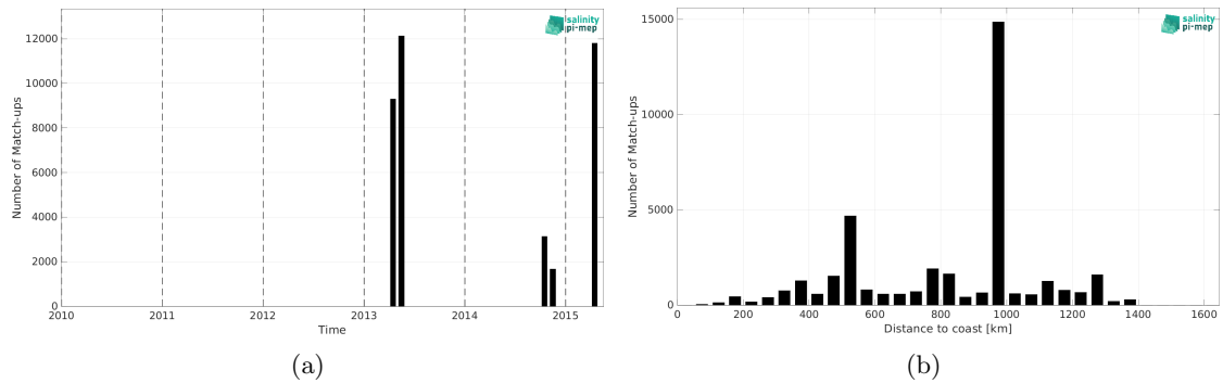
Figure 1: Number of match-ups between TSG (CSIC-UTM) and Aquarius SSS L3 CAP v5 - Monthly (JPL) SSS as a function of time (a) and as function of the distance to coast (b) over the Equatorial Ocean 10N-10S Pi-MEP region and for the full satellite product period.
