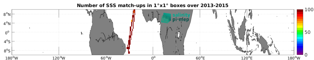
Figure 4: Number of SSS match-ups between TSG (CSIC-UTM) SSS and the Aquarius SSS L3 CAP v5 - Monthly (JPL) SSS product for the Equatorial Ocean 10N-10S Pi-MEP region over 1^\circ \times 1^\circ boxes and for the full satellite product period.
