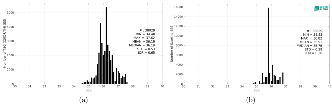
Figure 2: Histograms of SSS from TSG (CSIC-UTM) (a) and Aquarius SSS L3 CAP v5 - Monthly (JPL) (b) considering all match-up pairs per bins of 0.1 over the Equatorial Ocean 10N-10S Pi-MEP region and for the full satellite product period.
