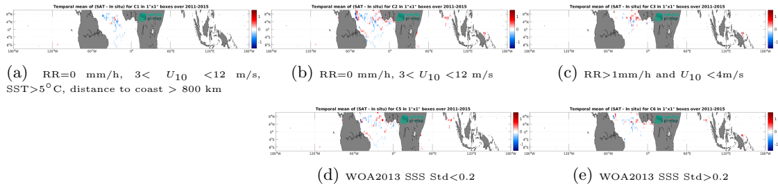
Figure 13: Temporal mean gridded over spatial boxes of size 1^\circ \times 1^\circ of \Delta SSS (Aquarius SSS L3 CAP v5 - Monthly (JPL) - Surface drifters) for 5 different subdatasets corresponding to:RR=0 mm/h, 3 < U_{10} < 12 m/s, SST>5°C, distance to coast > 800 km (a), RR=0 mm/h, 3 < U_{10} < 12 m/s (b), RR>1mm/h and U_{10} < 4 m/s (c), WOA2013 SSS Std<0.2 (d), WOA2013 SSS Std>0.2 (e).
