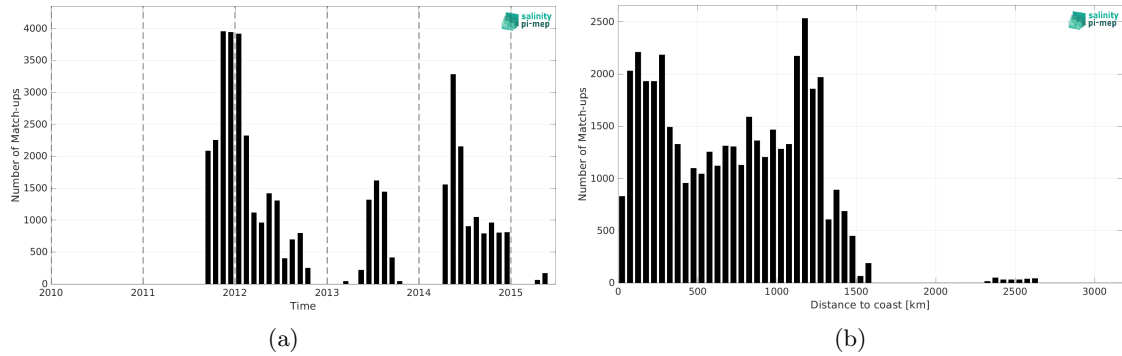
Figure 2: Number of match-ups between Surface drifters and Aquarius SSS L3 CAP v5 - Monthly (JPL) SSS as a function of time (a) and as function of the distance to coast (b) over the Equatorial Ocean 10N-10S Pi-MEP region and for the full satellite product period.
