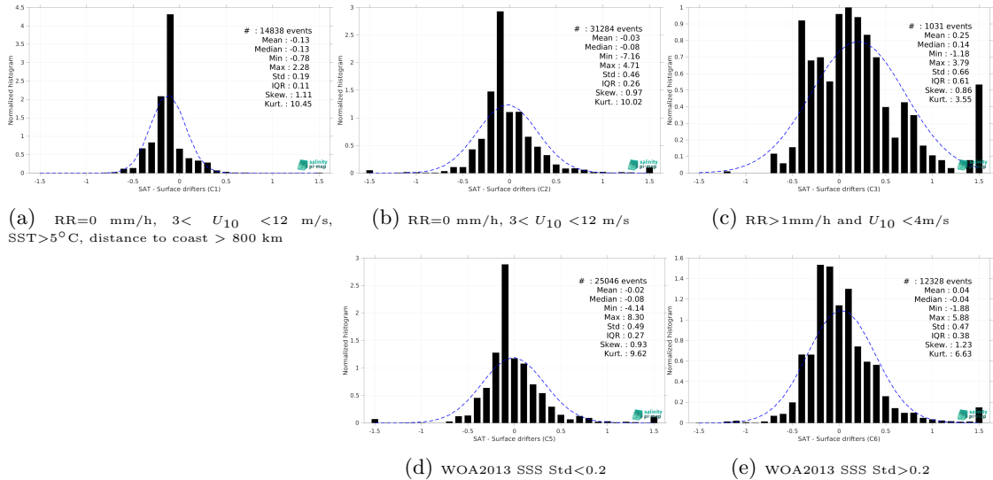
Figure 14: Normalized histogram of \Delta SSS (Aquarius SSS L3 CAP v5 - Monthly (JPL) - Surface drifters) for 5 different subdatasets corresponding to: RR=0 mm/h, 3 < U_{10} < 12 m/s, SST>5°C, distance to coast > 800 km (a), RR=0 mm/h, 3 < U_{10} < 12 m/s (b), RR>1mm/h and U_{10} < 4 m/s (c), WOA2013 SSS Std<0.2 (d), WOA2013 SSS Std>0.2 (e).
