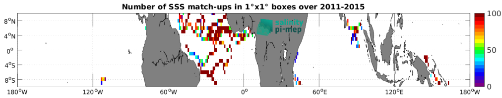
Figure 4: Number of SSS match-ups between Surface drifters SSS and the Aquarius SSS L3 CAP v5 - Monthly (JPL) SSS product for the Equatorial Ocean 10N-10S Pi-MEP region over 1^\circ \times 1^\circ boxes and for the full satellite product period.
