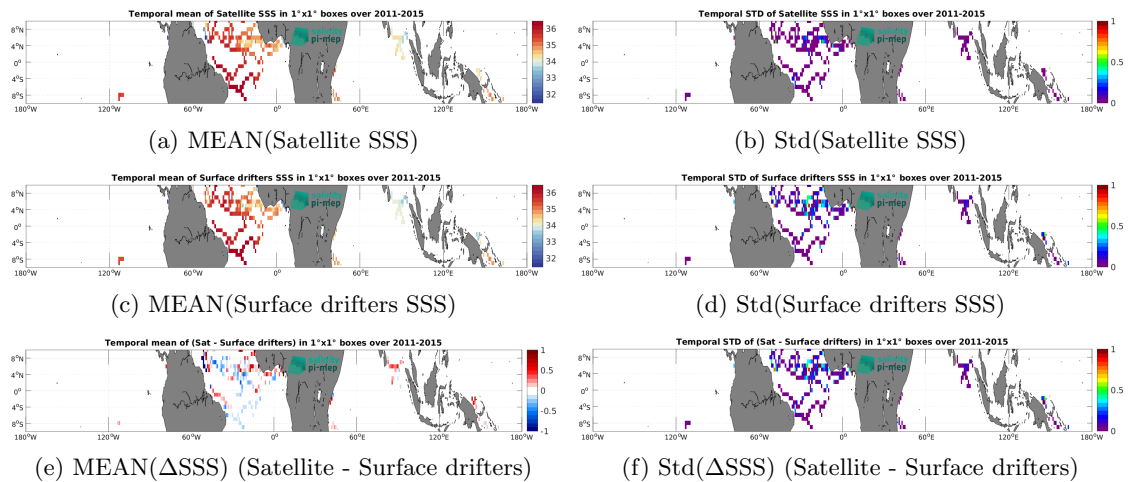
Figure 6: Temporal mean (left) and Std (right) of SSS from Aquarius SSS L3 CAP v5 - Monthly (JPL) (top), Surface drifters (middle), and of \Delta SSS (Satellite - Surface drifters). Only match-up pairs are used to generate these maps.
