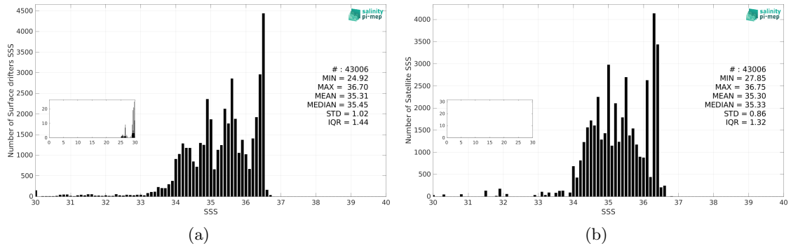
Figure 3: Histograms of SSS from Surface drifters (a) and Aquarius SSS L3 CAP v5 - Monthly (JPL) (b) considering all match-up pairs per bins of 0.1 over the Equatorial Ocean 10N-10S Pi-MEP region and for the full satellite product period.
