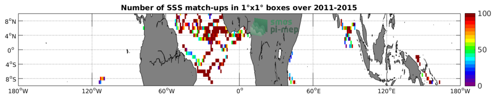
Figure 3: Number of SSS match-ups between Surface drifters SSS and the Aquarius-L3-JPL-V5-MONTHLY SSS product for the Equatorial Ocean 10N-10S Pi-MEP region over 1^\circ \times 1^\circ boxes and for the full satellite product period.
