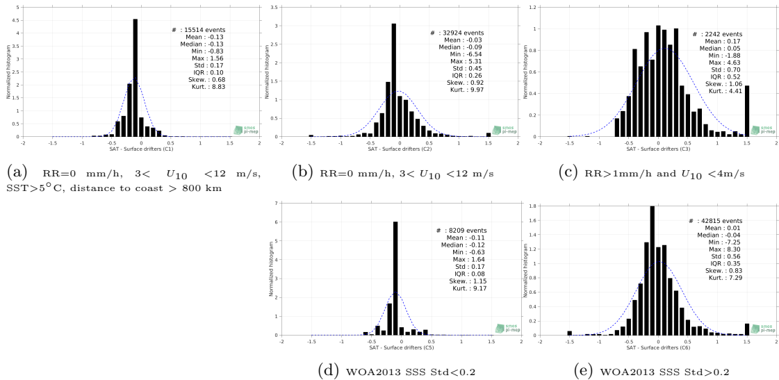
Figure 12: Normalized histogram of ΔSSS (Aquarius-L3-JPL-V5-MONTHLY - Surface drifters) for 5 different subdatasets corresponding to: RR=0 mm/h, 3 < U 10 < 12 m/s, SST > 5°C, distance to coast > 800 km (a), RR=0 mm/h, 3 < U 10 < 12 m/s (b), RR > 1mm/h and U 10 < 4m/s (c), WOA2013 SSS Std < 0.2 (d), WOA2013 SSS Std > 0.2 (e).
