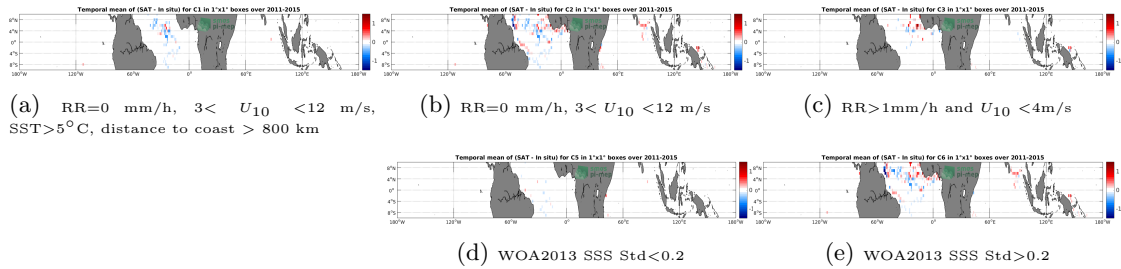
Figure 11: Temporal mean gridded over spatial boxes of size 1°x1° of ΔSSS (Aquarius-L3-JPL-V5-MONTHLY - Surface drifters) for 5 different subdatasets corresponding to:RR=0 mm/h, 3 < U 10 < 12 m/s, SST > 5°C, distance to coast > 800 km (a), RR=0 mm/h, 3 < U 10 < 12 m/s (b), RR > 1mm/h and U 10 < 4m/s (c), WOA2013 SSS Std < 0.2 (d), WOA2013 SSS Std > 0.2 (e).
