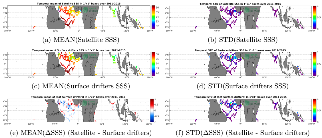
Figure 5: Temporal mean (left) and STD (right) of SSS from Aquarius-L3-JPL-V5-MONTHLY (top), Surface drifters (middle), and of \Delta SSS (Satellite - Surface drifters). Only match-up pairs are used to generate these maps.
