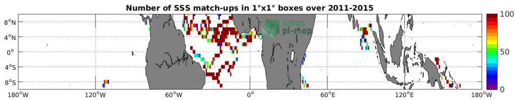
Figure 3: Number of SSS match-ups between Surface drifters SSS and the Aquarius-L3-JPL-V5-MONTHLY SSS product for the Equatorial Ocean 10N-10S Pi-MEP region over 1°x1° boxes and for the full satellite product period.
