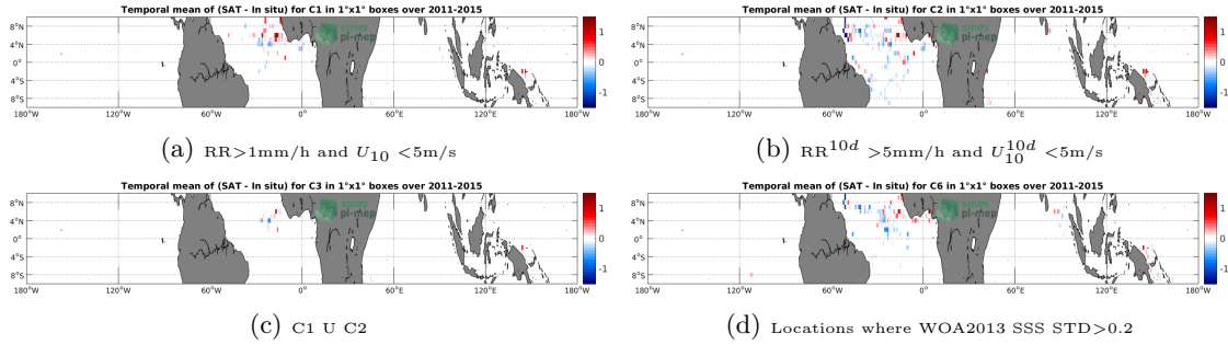
Figure 11: Temporal mean gridded over spatial boxes of size 1^\circ \times 1^\circ of \Delta SSS (Aquarius-L3-JPL-V5-MONTHLY - Surface drifters) for 4 different subdatasets corresponding to: RR > 1\text{mm/h} and U_{10} < 5\text{m/s} (a), RR^{10d} > 5\text{mm/h} and U_{10}^{10d} < 5\text{m/s} (b), C1 U C2 (c), Locations where WOA2013 SSS STD > 0.2 (d).
