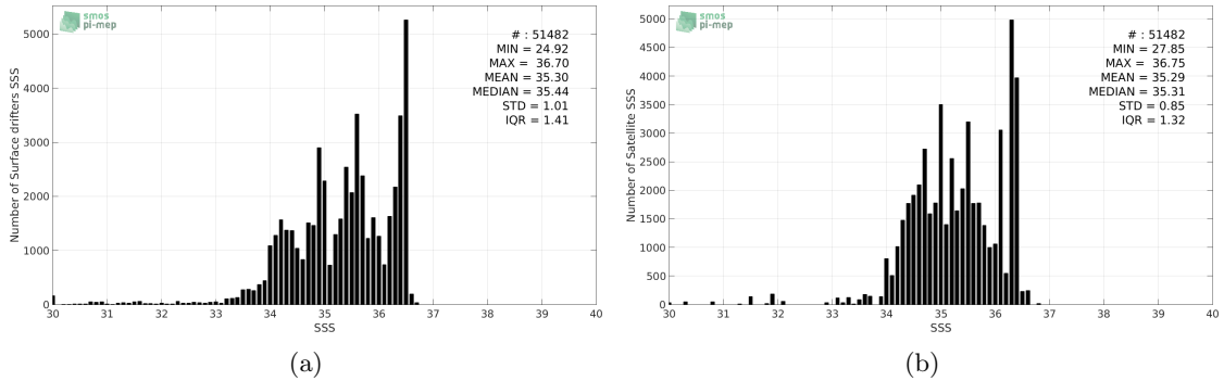
Figure 2: Histograms of SSS from Surface drifters (a) and Aquarius-L3-JPL-V5-MONTHLY (b) considering all match-up pairs per bins of 0.1 over the Equatorial Ocean 10N-10S Pi-MEP region and for the full satellite product period.
