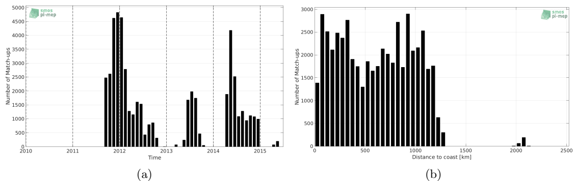
Figure 1: Number of match-ups between Surface drifters and Aquarius-L3-JPL-V5-MONTHLY SSS as a function of time (a) and as function of the distance to coast (b) over the Equatorial Ocean 10N-10S Pi-MEP region and for the full satellite product period.
