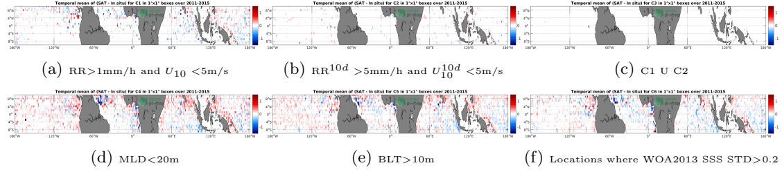
Figure 12: Temporal mean gridded over spatial boxes of size 1^\circ \times 1^\circ of \Delta SSS (Aquarius-L3-JPL-V5-MONTHLY - Argo) for 6 different subdatasets corresponding to: RR > 1\text{mm/h} and U_{10} < 5\text{m/s} (a), RR^{10d} > 5\text{mm/h} and U_{10}^{10d} < 5\text{m/s} (b), C1 U C2 (c), MLD < 20\text{m} (d), BLT > 10\text{m} (e), Locations where WOA2013 SSS STD > 0.2 (f).
