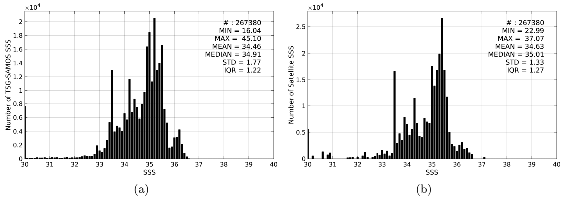
Figure 2: Histograms of SSS from TSG-SAMOS (a) and Aquarius-L3-JPL-V4-7DAY-RUNNING (b) considering all match-up pairs per bins of 0.1 over the Equatorial Ocean 10N-10S Pi-MEP region and for the full satellite product period.
