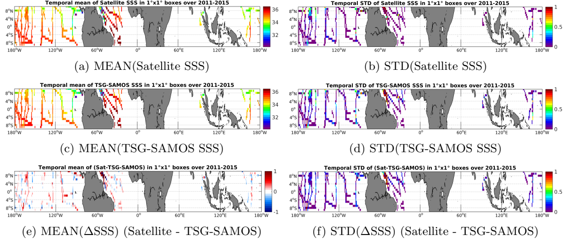
Figure 6: Temporal mean (left) and STD (right) of SSS from Aquarius-L3-JPL-V4-7DAY-RUNNING (top), TSG-SAMOS (middle), and of \Delta SSS (Satellite - TSG-SAMOS). Only match-up pairs are used to generate these maps.
