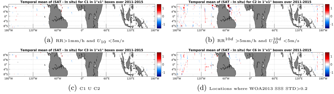
Figure 12: Temporal mean gridded over spatial boxes of size 1^\circ \times 1^\circ of \Delta SSS (Aquarius-L3-JPL-V4-7DAY-RUNNING - TSG-SAMOS) for 4 different subdatasets corresponding to: RR > 1 mm/h and U_{10} < 5 m/s (a), RR^{10d} > 5 mm/h and U_{10}^{10d} < 5 m/s (b), C1 U C2 (c), Locations where WOA2013 SSS STD > 0.2 (d).
