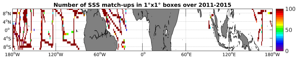
Figure 4: Number of SSS match-ups between TSG-SAMOS SSS and the Aquarius-L3-JPL-V4-7DAY-RUNNING SSS product for the Equatorial Ocean 10N-10S Pi-MEP region over 1^\circ \times 1^\circ boxes and for the full satellite product period.
