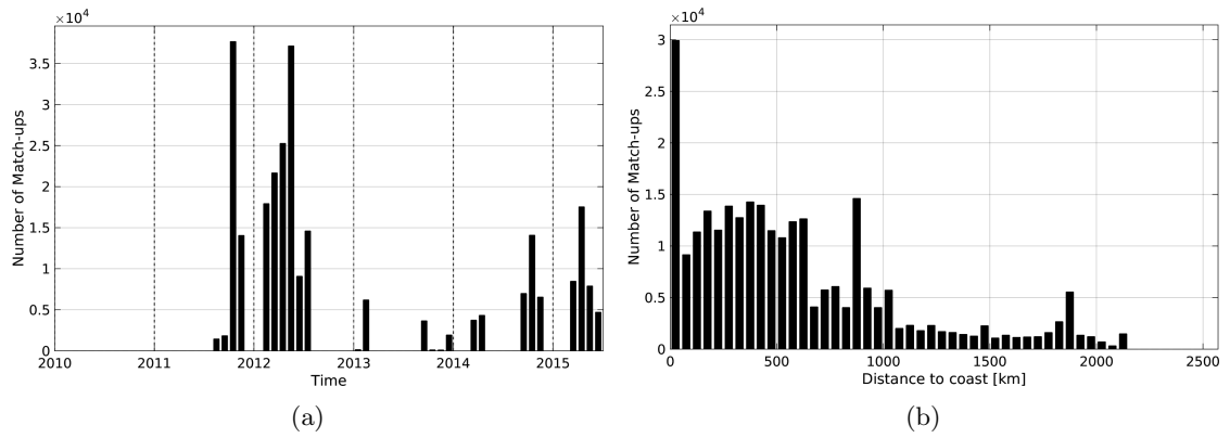
Figure 1: Number of match-ups between TSG-SAMOS and Aquarius-L3-JPL-V4-7DAY-RUNNING SSS as a function of time (a) and as function of the distance to coast (b) over the Equatorial Ocean 10N-10S Pi-MEP region and for the full satellite product period.
