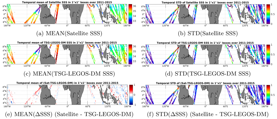
Figure 6: Temporal mean (left) and STD (right) of SSS from Aquarius-L3-JPL-V4-7DAY-RUNNING (top), TSG-LEGOS-DM (middle), and of \Delta SSS (Satellite - TSG-LEGOS-DM). Only match-up pairs are used to generate these maps.
