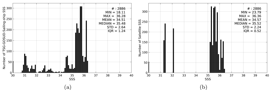
Figure 2: Histograms of SSS from TSG-GOSUD-Sailing-ship (a) and Aquarius-L3-JPL-V4-7DAY-RUNNING (b) considering all match-up pairs per bins of 0.1 over the Equatorial Ocean 10N-10S Pi-MEP region and for the full satellite product period.
