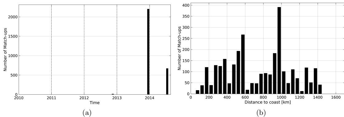
Figure 1: Number of match-ups between TSG-GOSUD-Sailing-ship and Aquarius-L3-JPL-V4-7DAY-RUNNING SSS as a function of time (a) and as function of the distance to coast (b) over the Equatorial Ocean 10N-10S Pi-MEP region and for the full satellite product period.
