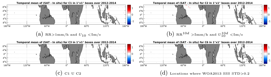
Figure 12: Temporal mean gridded over spatial boxes of size 1^\circ \times 1^\circ of \Delta SSS (Aquarius-L3-JPL-V4-7DAY-RUNNING - TSG-GOSUD-Sailing-ship) for 4 different subdatasets corresponding to: RR > 1\text{mm/h} and U_{10} < 5\text{m/s} (a), RR^{10d} > 5\text{mm/h} and U_{10}^{10d} < 5\text{m/s} (b), C1 U C2 (c), Locations where WOA2013 SSS STD > 0.2 (d).
