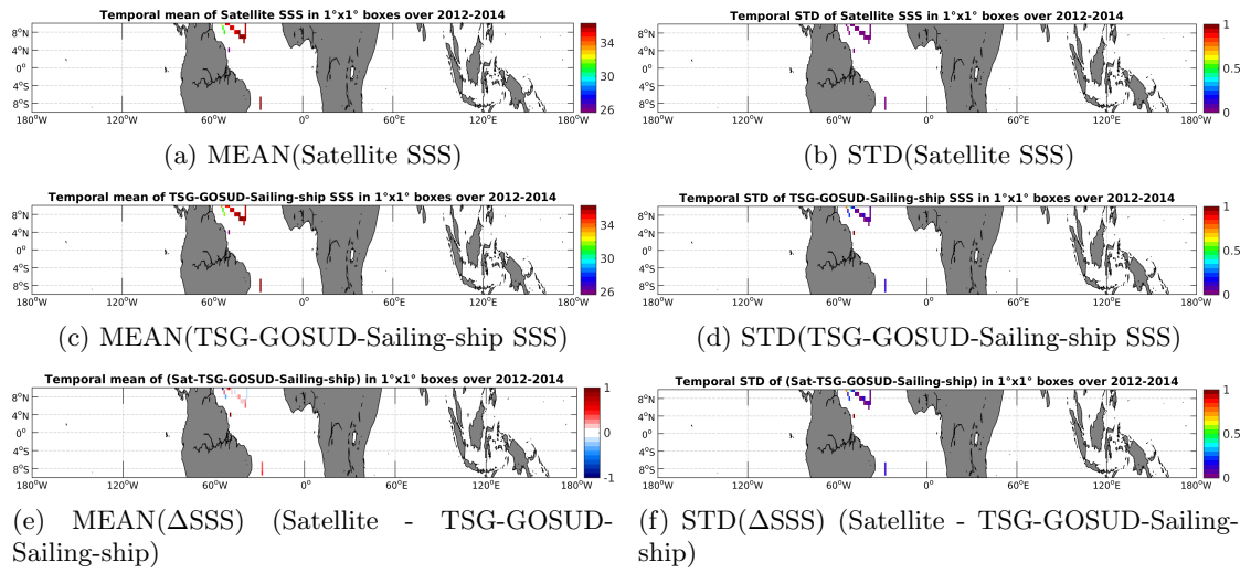
Figure 6: Temporal mean (left) and STD (right) of SSS from Aquarius-L3-JPL-V4-7DAY-RUNNING (top), TSG-GOSUD-Sailing-ship (middle), and of \Delta SSS (Satellite - TSG-GOSUD-Sailing-ship). Only match-up pairs are used to generate these maps.
