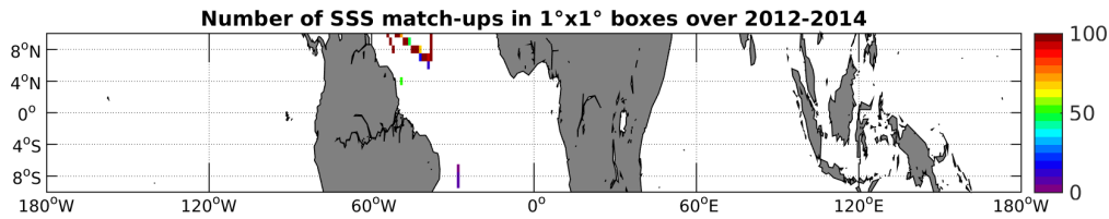
Figure 4: Number of SSS match-ups between TSG-GOSUD-Sailing-ship SSS and the Aquarius-L3-JPL-V4-7DAY-RUNNING SSS product for the Equatorial Ocean 10N-10S Pi-MEP region over 1°x1° boxes and for the full satellite product period.
