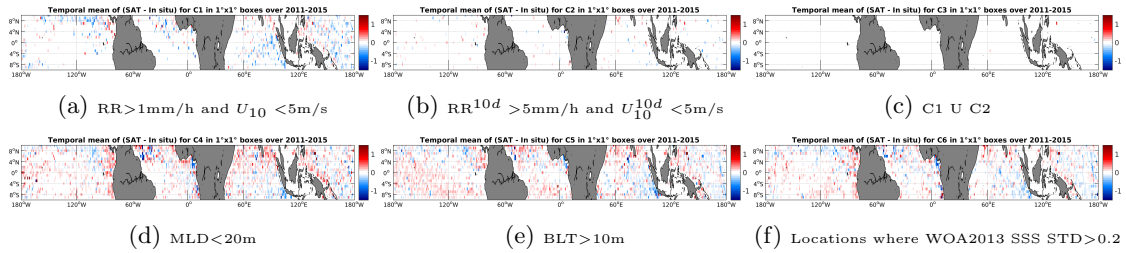
Figure 12: Temporal mean gridded over spatial boxes of size 1^\circ \times 1^\circ of \Delta SSS (Aquarius-L3-JPL-V4-7DAY-RUNNING - Argo) for 6 different subdatasets corresponding to: RR > 1\text{mm/h} and U_{10} < 5\text{m/s} (a), RR^{10d} > 5\text{mm/h} and U_{10}^{10d} < 5\text{m/s} (b), C1 U C2 (c), MLD < 20\text{m} (d), BLT > 10\text{m} (e), Locations where WOA2013 SSS STD > 0.2 (f).
