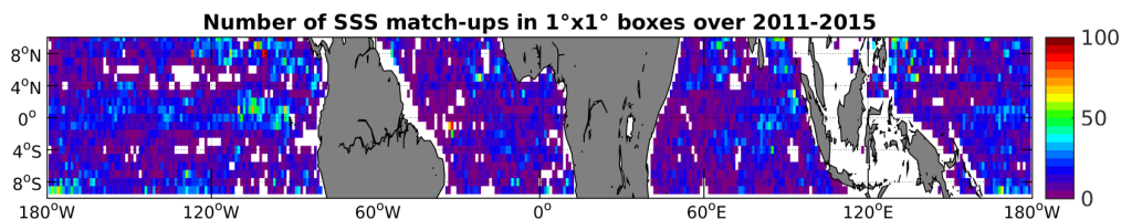
Figure 4: Number of SSS match-ups between Argo SSS and the Aquarius-L3-JPL-V4-7DAY-RUNNING SSS product for the Equatorial Ocean 10N-10S Pi-MEP region over 1^\circ \times 1^\circ boxes and for the full satellite product period.
