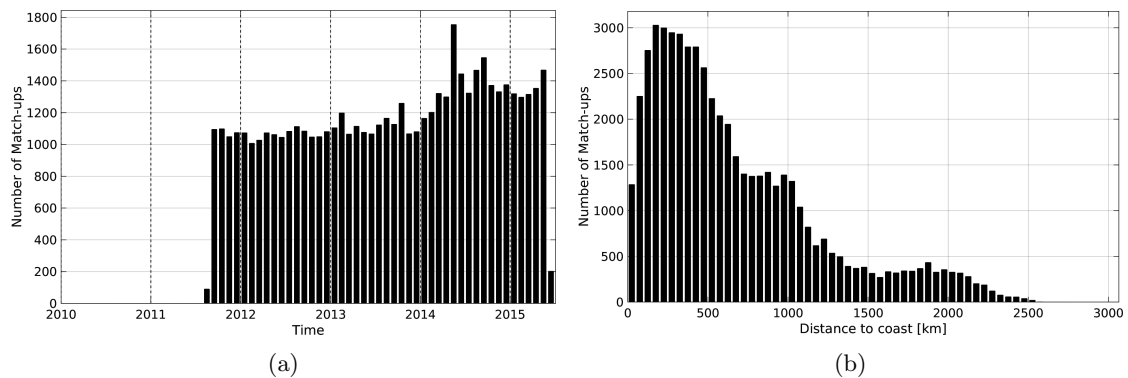
Figure 1: Number of match-ups between Argo and Aquarius-L3-JPL-V4-7DAY-RUNNING SSS as a function of time (a) and as function of the distance to coast (b) over the Equatorial Ocean 10N-10S Pi-MEP region and for the full satellite product period.
