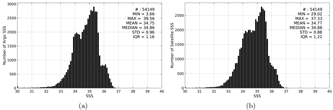
Figure 2: Histograms of SSS from Argo (a) and Aquarius-L3-JPL-V4-7DAY-RUNNING (b) considering all match-up pairs per bins of 0.1 over the Equatorial Ocean 10N-10S Pi-MEP region and for the full satellite product period.
