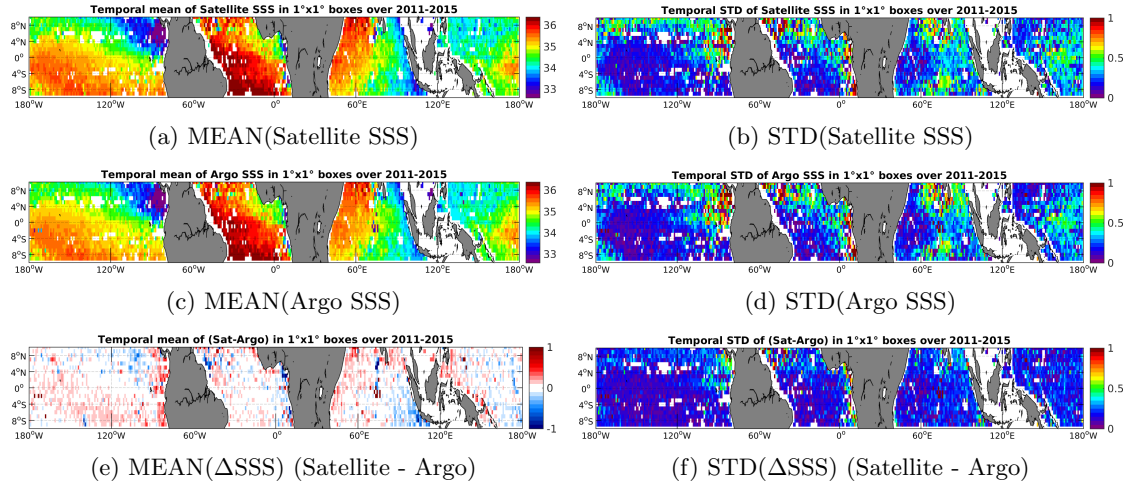
Figure 6: Temporal mean (left) and STD (right) of SSS from Aquarius-L3-JPL-V4-7DAY-RUNNING (top), Argo (middle), and of \Delta SSS (Satellite - Argo). Only match-up pairs are used to generate these maps.
