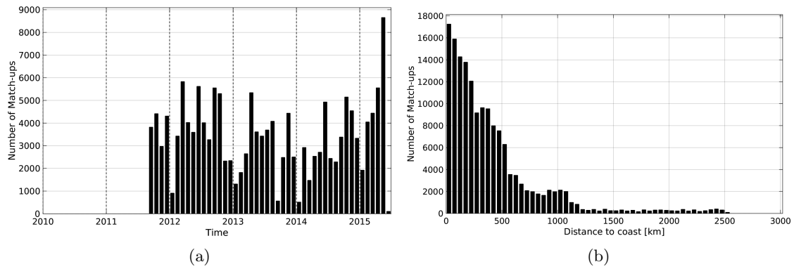
Figure 1: Number of match-ups between TSG-LEGOS-DM and Aquarius-L3-JPL-V4-MONTHLY SSS as a function of time (a) and as function of the distance to coast (b) over the Equatorial Ocean 10N-10S Pi-MEP region and for the full satellite product period.
