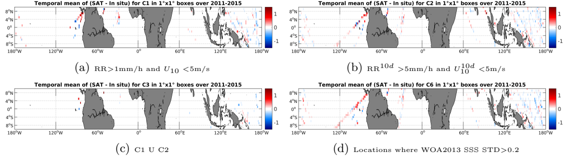
Figure 12: Temporal mean gridded over spatial boxes of size 1^\circ \times 1^\circ of \Delta SSS (Aquarius-L3-JPL-V4-MONTHLY - TSG-LEGOS-DM) for 4 different subdatasets corresponding to: RR > 1\text{mm/h} and U_{10} < 5\text{m/s} (a), RR^{10d} > 5\text{mm/h} and U_{10}^{10d} < 5\text{m/s} (b), C1 U C2 (c), Locations where WOA2013 SSS STD > 0.2 (d).
