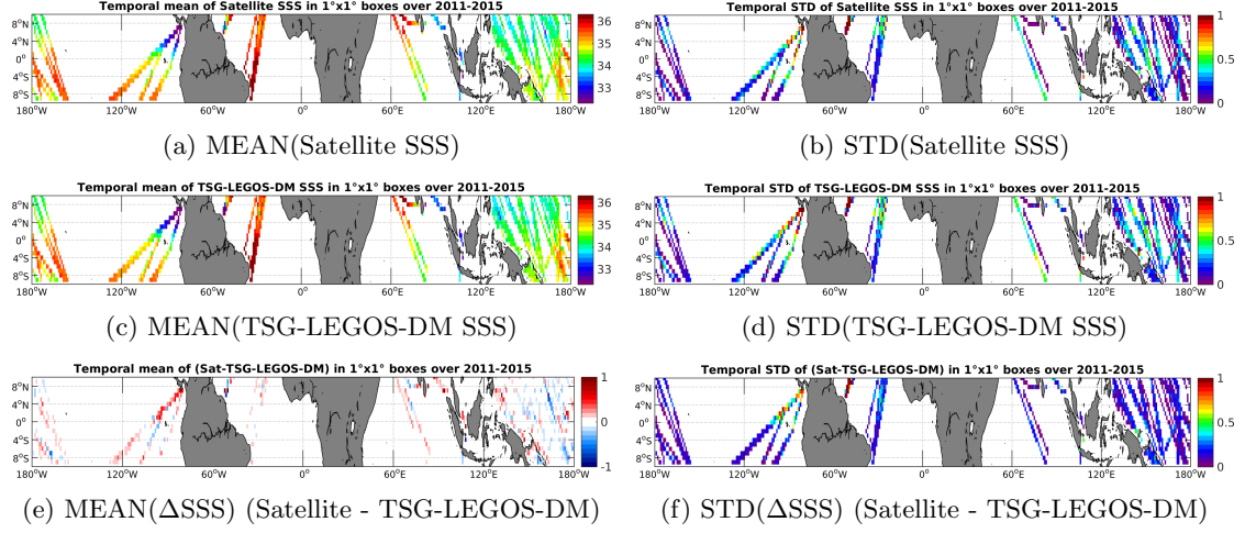
Figure 6: Temporal mean (left) and STD (right) of SSS from Aquarius-L3-JPL-V4-MONTHLY (top), TSG-LEGOS-DM (middle), and of \Delta SSS (Satellite - TSG-LEGOS-DM). Only match-up pairs are used to generate these maps.
