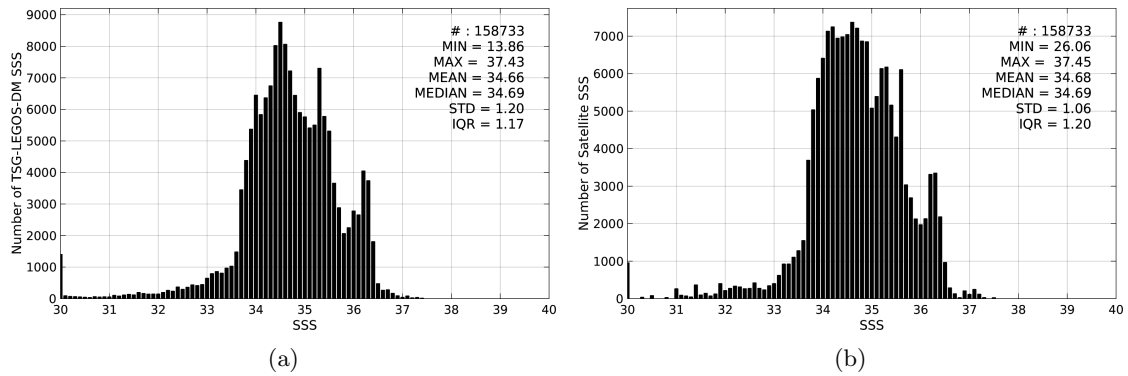
Figure 2: Histograms of SSS from TSG-LEGOS-DM (a) and Aquarius-L3-JPL-V4-MONTHLY (b) considering all match-up pairs per bins of 0.1 over the Equatorial Ocean 10N-10S Pi-MEP region and for the full satellite product period.
