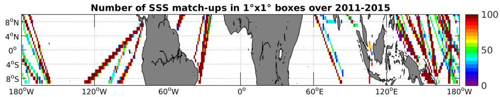
Figure 4: Number of SSS match-ups between TSG-LEGOS-DM SSS and the Aquarius-L3-JPL-V4-MONTHLY SSS product for the Equatorial Ocean 10N-10S Pi-MEP region over 1^\circ \times 1^\circ boxes and for the full satellite product period.
