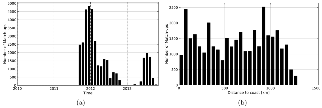
Figure 1: Number of match-ups between Surface drifters and Aquarius-L3-JPL-V4-MONTHLY SSS as a function of time (a) and as function of the distance to coast (b) over the Equatorial Ocean 10N-10S Pi-MEP region and for the full satellite product period.
