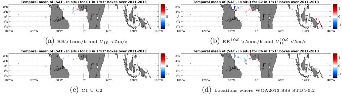
Figure 11: Temporal mean gridded over spatial boxes of size 1^\circ \times 1^\circ of \Delta SSS (Aquarius-L3-JPL-V4-MONTHLY - Surface drifters) for 4 different subdatasets corresponding to: RR > 1\text{mm/h} and U_{10} < 5\text{m/s} (a), RR^{10d} > 5\text{mm/h} and U_{10}^{10d} < 5\text{m/s} (b), C1 U C2 (c), Locations where WOA2013 SSS STD > 0.2 (d).
