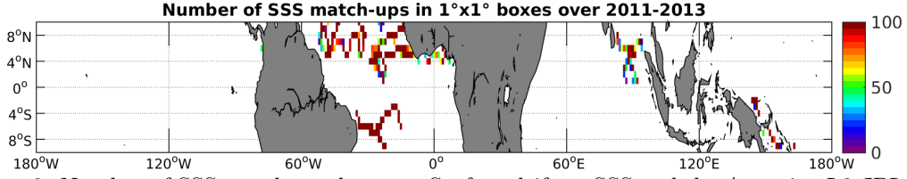
Figure 3: Number of SSS match-ups between Surface drifters SSS and the Aquarius-L3-JPL-V4-MONTHLY SSS product for the Equatorial Ocean 10N-10S Pi-MEP region over 1^\circ \times 1^\circ boxes and for the full satellite product period.
