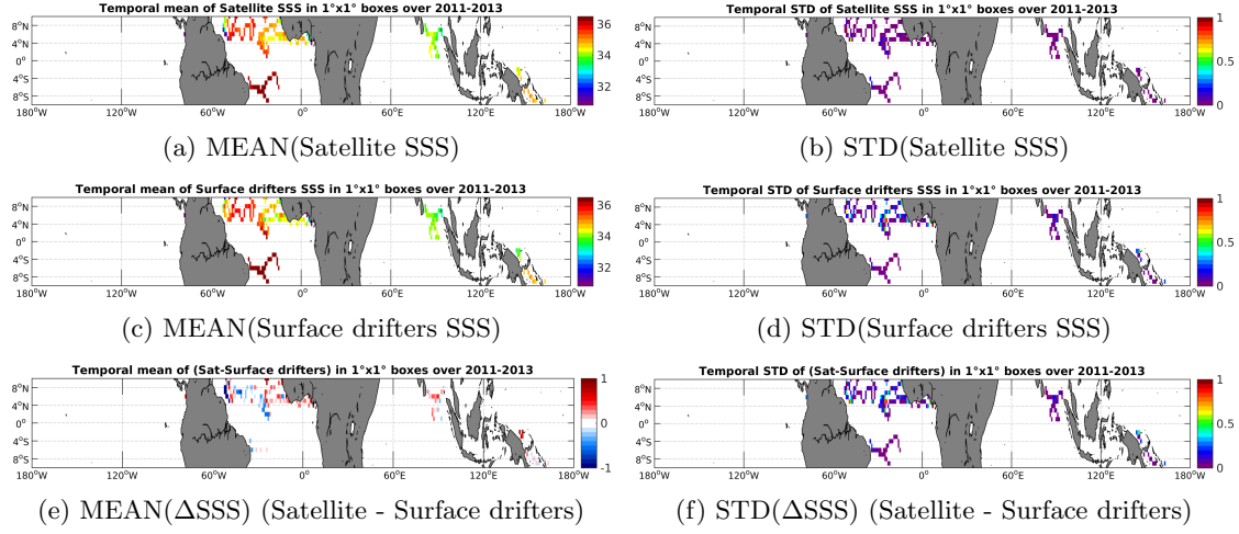
Figure 5: Temporal mean (left) and STD (right) of SSS from Aquarius-L3-JPL-V4-MONTHLY (top), Surface drifters (middle), and of \Delta SSS (Satellite - Surface drifters). Only match-up pairs are used to generate these maps.
