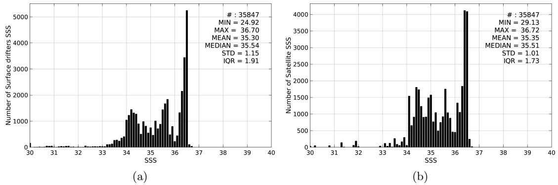
Figure 2: Histograms of SSS from Surface drifters (a) and Aquarius-L3-JPL-V4-MONTHLY (b) considering all match-up pairs per bins of 0.1 over the Equatorial Ocean 10N-10S Pi-MEP region and for the full satellite product period.
