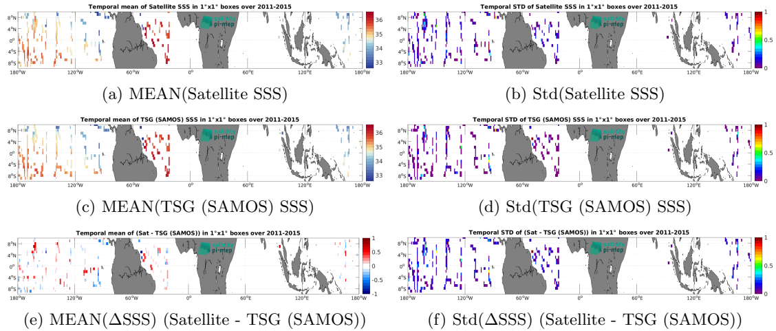
Figure 7: Temporal mean (left) and Std (right) of SSS from Aquarius SSS L2 OR v5 (NASA-GSFC) (top), TSG (SAMOS) (middle), and of \Delta SSS (Satellite - TSG (SAMOS)). Only match-up pairs are used to generate these maps.
