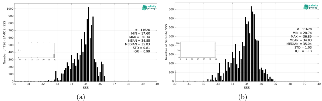
Figure 3: Histograms of SSS from TSG (SAMOS) (a) and Aquarius SSS L2 OR v5 (NASA-GSFC) (b) considering all match-up pairs per bins of 0.1 over the Equatorial Ocean 10N-10S Pi-MEP region and for the full satellite product period.
