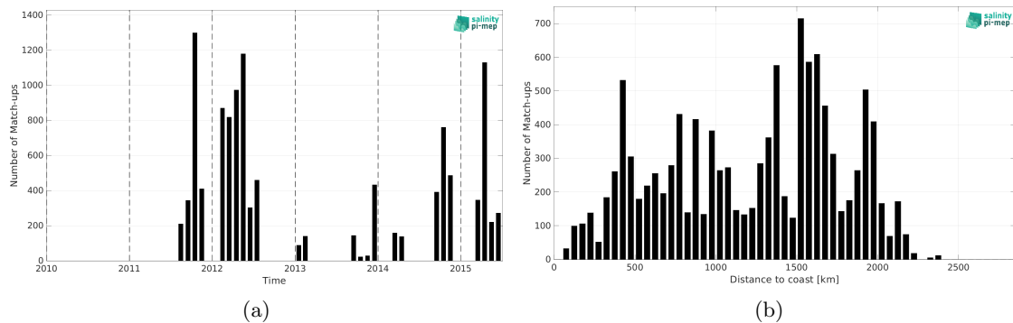
Figure 2: Number of match-ups between TSG (SAMOS) and Aquarius SSS L2 OR v5 (NASA-GSFC) SSS as a function of time (a) and as function of the distance to coast (b) over the Equatorial Ocean 10N-10S Pi-MEP region and for the full satellite product period.
