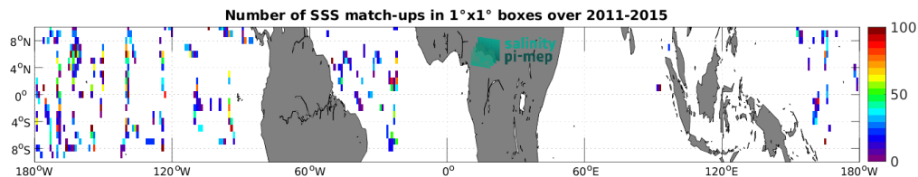
Figure 5: Number of SSS match-ups between TSG (SAMOS) SSS and the Aquarius SSS L2 OR v5 (NASA-GSFC) SSS product for the Equatorial Ocean 10N-10S Pi-MEP region over 1^\circ \times 1^\circ boxes and for the full satellite product period.
