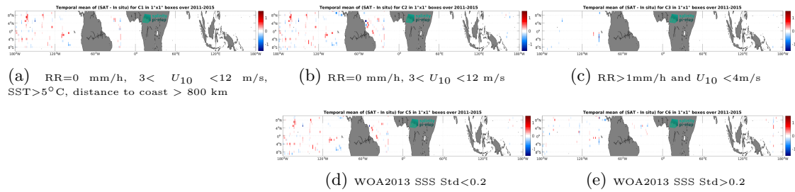
Figure 14: Temporal mean gridded over spatial boxes of size 1^\circ \times 1^\circ of \Delta SSS (Aquarius SSS L2 OR v5 (NASA-GSFC) - TSG (SAMOS)) for 5 different subdatasets corresponding to: RR=0 mm/h, 3 < U_{10} < 12 m/s, SST>5°C, distance to coast > 800 km (a), RR=0 mm/h, 3 < U_{10} < 12 m/s (b), RR>1mm/h and U_{10} < 4 m/s (c), WOA2013 SSS Std<0.2 (d), WOA2013 SSS Std>0.2 (e).
