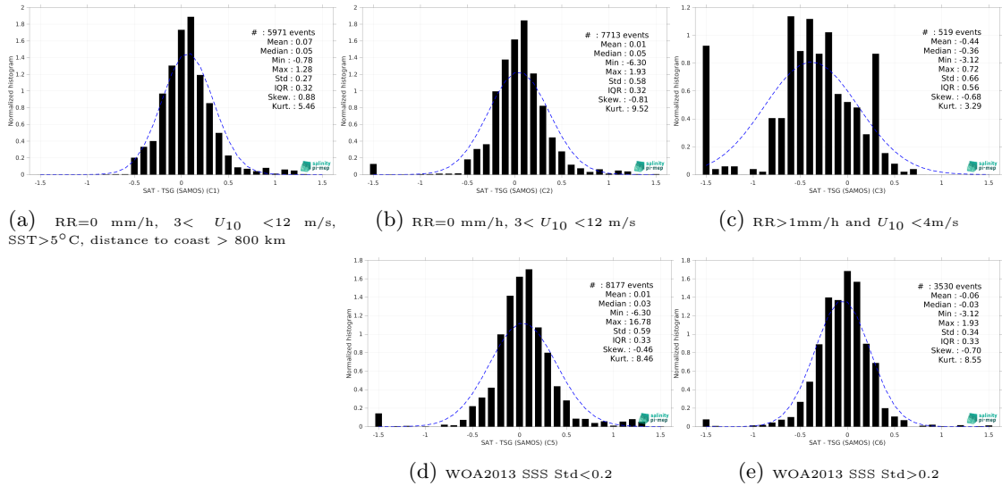
Figure 13: Normalized histogram of \Delta SSS (Aquarius SSS L2 OR v5 (NASA-GSFC) - TSG (SAMOS)) for 5 different subdatasets corresponding to: RR=0 mm/h, 3 < U_{10} < 12 m/s, SST >5^\circ C, distance to coast > 800 km (a), RR=0 mm/h, 3 < U_{10} < 12 m/s (b), RR >1 mm/h and U_{10} < 4 m/s (c), WOA2013 SSS Std <0.2 (d), WOA2013 SSS Std >0.2 (e).
