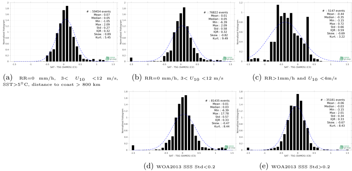
Figure 13: Normalized histogram of \Delta SSS (Aquarius SSS L2 OR v5 (NASA-GSFC) - TSG (SAMOS)) for 5 different subdatasets corresponding to: RR=0 mm/h, 3 < U_{10} < 12 m/s, SST >5^\circ\text{C} , distance to coast > 800 km (a), RR=0 mm/h, 3 < U_{10} < 12 m/s (b), RR >1 mm/h and U_{10} < 4 m/s (c), WOA2013 SSS Std <0.2 (d), WOA2013 SSS Std >0.2 (e).
