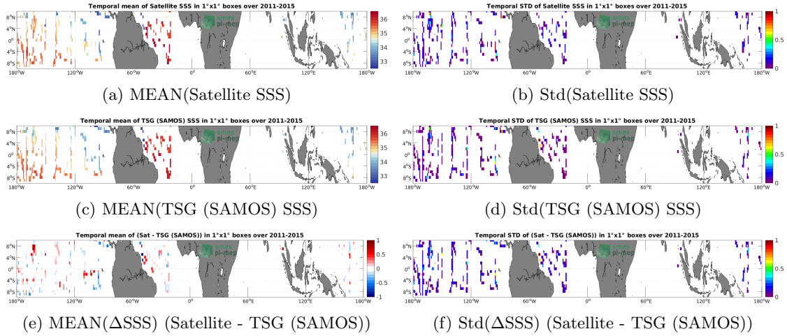
Figure 6: Temporal mean (left) and Std (right) of SSS from Aquarius SSS L2 OR v5 (NASA-GSFC) (top), TSG (SAMOS) (middle), and of \Delta SSS (Satellite - TSG (SAMOS)). Only match-up pairs are used to generate these maps.
