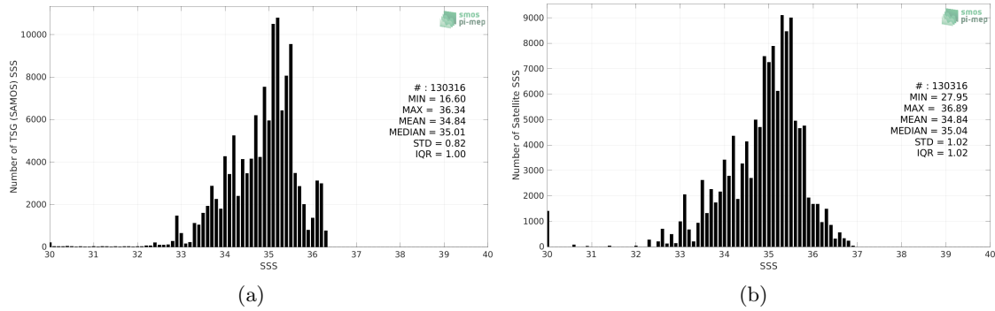
Figure 2: Histograms of SSS from TSG (SAMOS) (a) and Aquarius SSS L2 OR v5 (NASA-GSFC) (b) considering all match-up pairs per bins of 0.1 over the Equatorial Ocean 10N-10S Pi-MEP region and for the full satellite product period.
