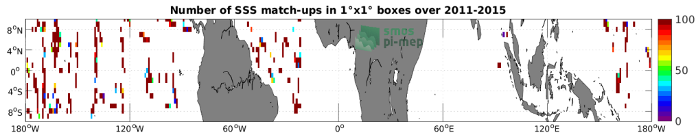
Figure 4: Number of SSS match-ups between TSG (SAMOS) SSS and the Aquarius SSS L2 OR v5 (NASA-GSFC) SSS product for the Equatorial Ocean 10N-10S Pi-MEP region over 1^\circ \times 1^\circ boxes and for the full satellite product period.
