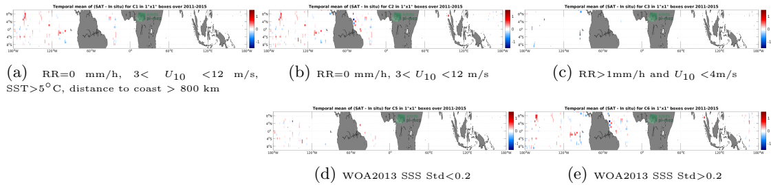
Figure 12: Temporal mean gridded over spatial boxes of size 1^\circ \times 1^\circ of \Delta SSS (Aquarius SSS L2 OR v5 (NASA-GSFC) - TSG (SAMOS)) for 5 different subdatasets corresponding to: RR=0 mm/h, 3 < U_{10} < 12 m/s, SST>5°C, distance to coast > 800 km (a), RR=0 mm/h, 3 < U_{10} < 12 m/s (b), RR>1mm/h and U_{10} < 4 m/s (c), WOA2013 SSS Std<0.2 (d), WOA2013 SSS Std>0.2 (e).
