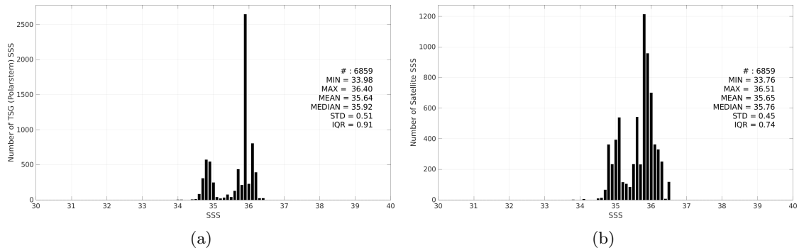
Figure 3: Histograms of SSS from TSG (Polarstern) (a) and Aquarius SSS L2 OR v5 (NASA-GSFC) (b) considering all match-up pairs per bins of 0.1 over the Equatorial Ocean 10N-10S Pi-MEP region and for the full satellite product period.
