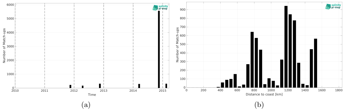
Figure 2: Number of match-ups between TSG (Polarstern) and Aquarius SSS L2 OR v5 (NASA-GSFC) SSS as a function of time (a) and as function of the distance to coast (b) over the Equatorial Ocean 10N-10S Pi-MEP region and for the full satellite product period.
