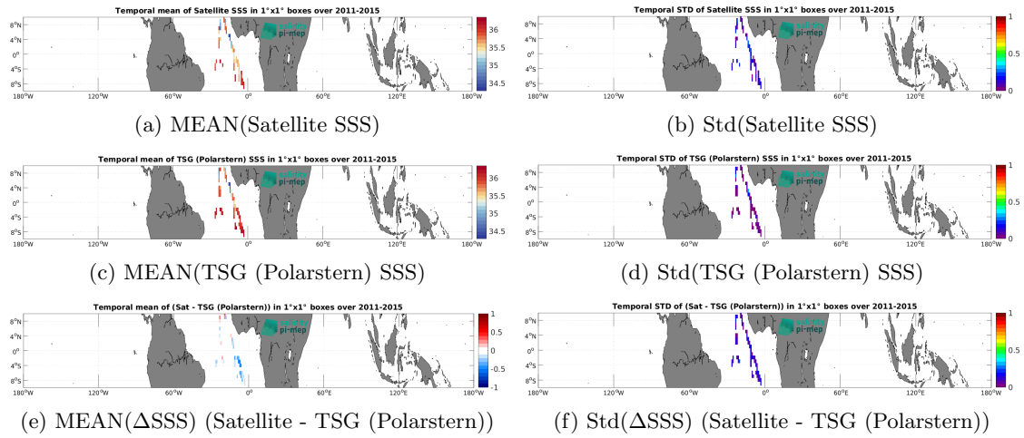
Figure 7: Temporal mean (left) and Std (right) of SSS from Aquarius SSS L2 OR v5 (NASA-GSFC) (top), TSG (Polarstern) (middle), and of \Delta SSS (Satellite - TSG (Polarstern)). Only match-up pairs are used to generate these maps.
