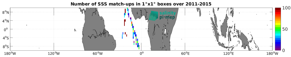
Figure 5: Number of SSS match-ups between TSG (Polarstern) SSS and the Aquarius SSS L2 OR v5 (NASA-GSFC) SSS product for the Equatorial Ocean 10N-10S Pi-MEP region over 1^\circ \times 1^\circ boxes and for the full satellite product period.
