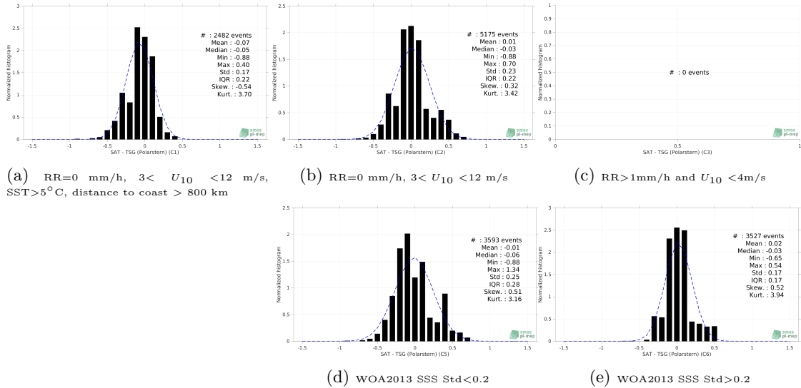
Figure 13: Normalized histogram of \Delta SSS (Aquarius SSS L2 OR v5 (NASA-GSFC) - TSG (Polarstern)) for 5 different subdatasets corresponding to: RR=0 mm/h, 3 < U_{10} < 12 m/s, SST > 5^\circ C , distance to coast > 800 km (a), RR=0 mm/h, 3 < U_{10} < 12 m/s (b), RR>1mm/h and U_{10} < 4 m/s (c), WOA2013 SSS Std<0.2 (d), WOA2013 SSS Std>0.2 (e).
