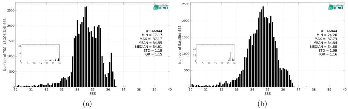
Figure 3: Histograms of SSS from TSG (LEGOS-DM) (a) and Aquarius SSS L2 OR v5 (NASA-GSFC) (b) considering all match-up pairs per bins of 0.1 over the Equatorial Ocean 10N-10S Pi-MEP region and for the full satellite product period.
