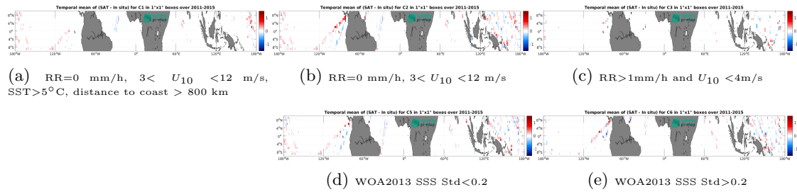
Figure 14: Temporal mean gridded over spatial boxes of size 1^\circ \times 1^\circ of \Delta SSS (Aquarius SSS L2 OR v5 (NASA-GSFC) - TSG (LEGOS-DM)) for 5 different subdatasets corresponding to:RR=0 mm/h, 3 < U_{10} < 12 m/s, SST>5°C, distance to coast > 800 km (a), RR=0 mm/h, 3 < U_{10} < 12 m/s (b), RR>1mm/h and U_{10} < 4 m/s (c), WOA2013 SSS Std<0.2 (d), WOA2013 SSS Std>0.2 (e).
