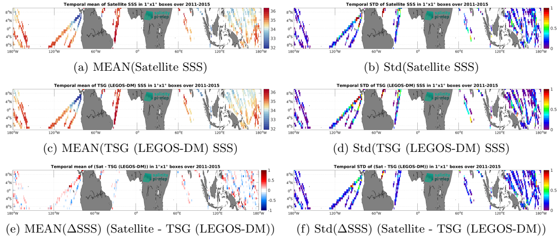
Figure 7: Temporal mean (left) and Std (right) of SSS from Aquarius SSS L2 OR v5 (NASA-GSFC) (top), TSG (LEGOS-DM) (middle), and of \Delta SSS (Satellite - TSG (LEGOS-DM)). Only match-up pairs are used to generate these maps.
