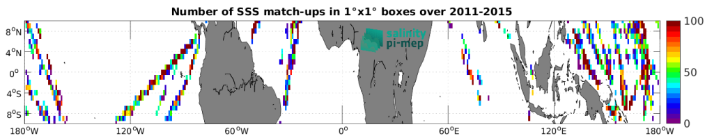
Figure 5: Number of SSS match-ups between TSG (LEGOS-DM) SSS and the Aquarius SSS L2 OR v5 (NASA-GSFC) SSS product for the Equatorial Ocean 10N-10S Pi-MEP region over 1^\circ \times 1^\circ boxes and for the full satellite product period.
