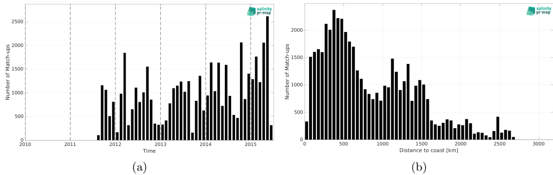
Figure 2: Number of match-ups between TSG (LEGOS-DM) and Aquarius SSS L2 OR v5 (NASA-GSFC) SSS as a function of time (a) and as function of the distance to coast (b) over the Equatorial Ocean 10N-10S Pi-MEP region and for the full satellite product period.
