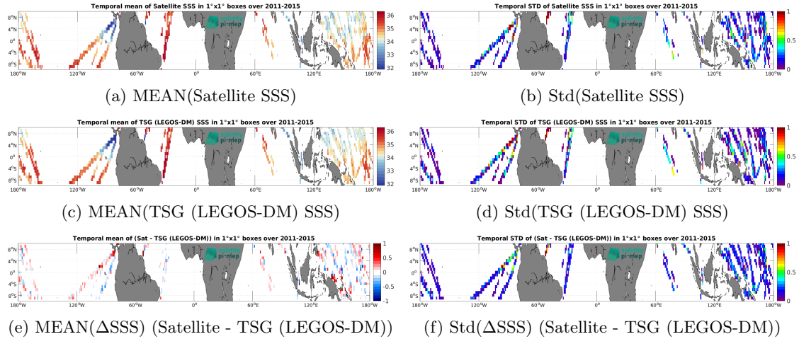
Figure 6: Temporal mean (left) and Std (right) of SSS from Aquarius SSS L2 OR v5 (NASA-GSFC) (top), TSG (LEGOS-DM) (middle), and of \Delta SSS (Satellite - TSG (LEGOS-DM)). Only match-up pairs are used to generate these maps.
