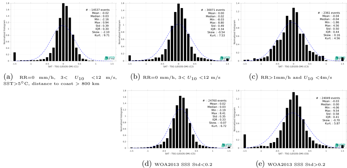
Figure 13: Normalized histogram of \Delta SSS (Aquarius SSS L2 OR v5 (NASA-GSFC) - TSG (LEGOS-DM)) for 5 different subdatasets corresponding to: RR=0 mm/h, 3 < U_{10} < 12 m/s, SST >5^\circ\text{C} , distance to coast > 800 km (a), RR=0 mm/h, 3 < U_{10} < 12 m/s (b), RR >1 mm/h and U_{10} < 4 m/s (c), WOA2013 SSS Std <0.2 (d), WOA2013 SSS Std >0.2 (e).
