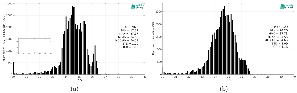
Figure 2: Histograms of SSS from TSG (LEGOS-DM) (a) and Aquarius SSS L2 OR v5 (NASA-GSFC) (b) considering all match-up pairs per bins of 0.1 over the Equatorial Ocean 10N-10S Pi-MEP region and for the full satellite product period.
