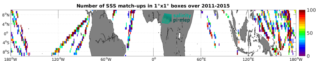
Figure 4: Number of SSS match-ups between TSG (LEGOS-DM) SSS and the Aquarius SSS L2 OR v5 (NASA-GSFC) SSS product for the Equatorial Ocean 10N-10S Pi-MEP region over 1^\circ \times 1^\circ boxes and for the full satellite product period.
