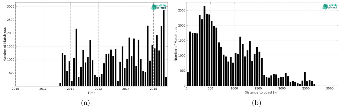
Figure 1: Number of match-ups between TSG (LEGOS-DM) and Aquarius SSS L2 OR v5 (NASA-GSFC) SSS as a function of time (a) and as function of the distance to coast (b) over the Equatorial Ocean 10N-10S Pi-MEP region and for the full satellite product period.
