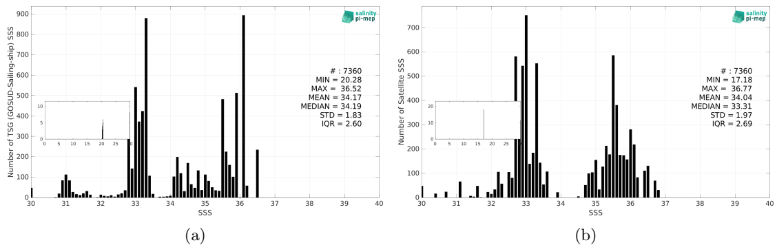
Figure 3: Histograms of SSS from TSG (GOSUD-Sailing-ship) (a) and Aquarius SSS L2 OR v5 (NASA-GSFC) (b) considering all match-up pairs per bins of 0.1 over the Equatorial Ocean 10N-10S Pi-MEP region and for the full satellite product period.
