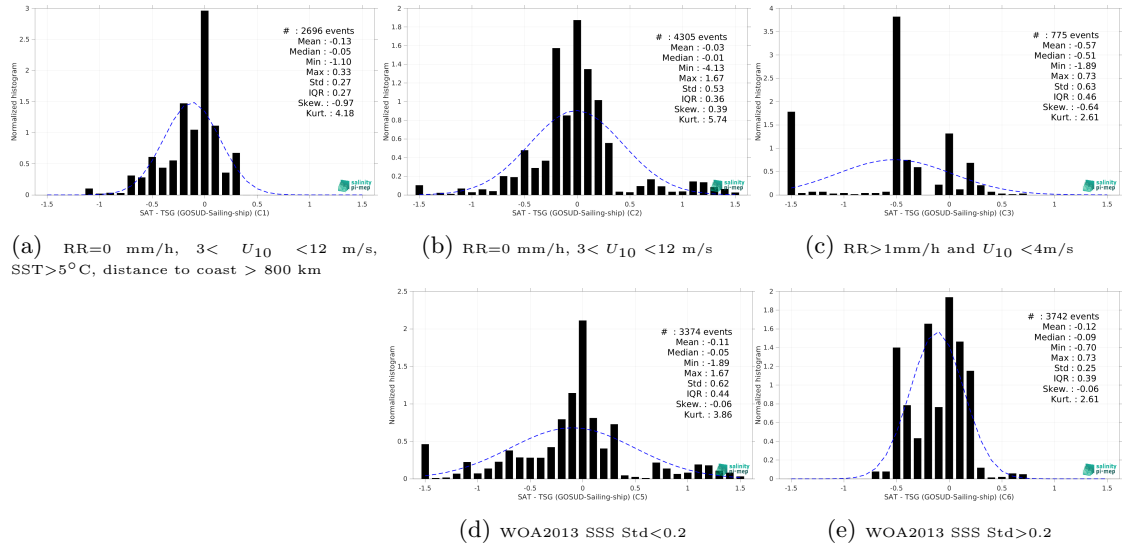
Figure 15: Normalized histogram of \Delta SSS (Aquarius SSS L2 OR v5 (NASA-GSFC) - TSG (GOSUD-Sailing-ship)) for 5 different subdatasets corresponding to: RR=0 mm/h, 3 < U_{10} < 12 m/s, SST >5^\circ\text{C} , distance to coast > 800 km (a), RR=0 mm/h, 3 < U_{10} < 12 m/s (b), RR >1 mm/h and U_{10} < 4 m/s (c), WOA2013 SSS Std <0.2 (d), WOA2013 SSS Std >0.2 (e).
