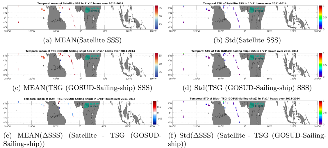
Figure 7: Temporal mean (left) and Std (right) of SSS from Aquarius SSS L2 OR v5 (NASA-GSFC) (top), TSG (GOSUD-Sailing-ship) (middle), and of \Delta SSS (Satellite - TSG (GOSUD-Sailing-ship)). Only match-up pairs are used to generate these maps.
