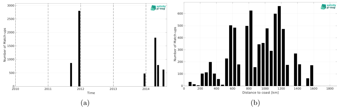
Figure 2: Number of match-ups between TSG (GOSUD-Sailing-ship) and Aquarius SSS L2 OR v5 (NASA-GSFC) SSS as a function of time (a) and as function of the distance to coast (b) over the Equatorial Ocean 10N-10S Pi-MEP region and for the full satellite product period.
