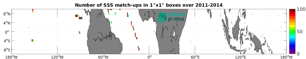
Figure 5: Number of SSS match-ups between TSG (GOSUD-Sailing-ship) SSS and the Aquarius SSS L2 OR v5 (NASA-GSFC) SSS product for the Equatorial Ocean 10N-10S Pi-MEP region over 1^\circ \times 1^\circ boxes and for the full satellite product period.
