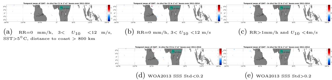
Figure 12: Temporal mean gridded over spatial boxes of size 1^\circ \times 1^\circ of \Delta\text{SSS} (Aquarius SSS L2 OR v5 (NASA-GSFC) - TSG (GOSUD-Sailing-ship)) for 5 different subdatasets corresponding to: RR=0 mm/h, 3 < U_{10} < 12 m/s, SST>5°C, distance to coast > 800 km (a), RR=0 mm/h, 3 < U_{10} < 12 m/s (b), RR>1mm/h and U_{10} < 4 m/s (c), WOA2013 SSS Std<0.2 (d), WOA2013 SSS Std>0.2 (e).
