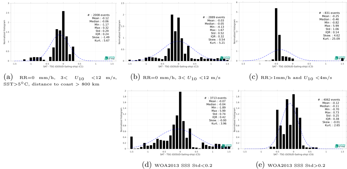
Figure 13: Normalized histogram of \Delta\text{SSS} (Aquarius SSS L2 OR v5 (NASA-GSFC) - TSG (GOSUD-Sailing-ship)) for 5 different subdatasets corresponding to: RR=0 mm/h, 3 < U_{10} < 12 m/s, SST>5°C, distance to coast > 800 km (a), RR=0 mm/h, 3 < U_{10} < 12 m/s (b), RR>1mm/h and U_{10} < 4 m/s (c), WOA2013 SSS Std<0.2 (d), WOA2013 SSS Std>0.2 (e).
