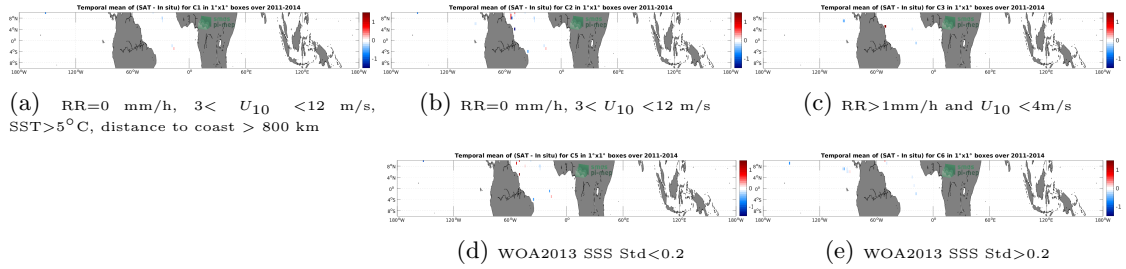
Figure 12: Temporal mean gridded over spatial boxes of size 1^\circ \times 1^\circ of \Delta SSS (Aquarius SSS L2 OR v5 (NASA-GSFC) - TSG (GOSUD-Sailing-ship)) for 5 different subdatasets corresponding to:RR=0 mm/h, 3 < U_{10} < 12 m/s, SST >5^\circ C, distance to coast > 800 km (a), RR=0 mm/h, 3 < U_{10} < 12 m/s (b), RR >1 mm/h and U_{10} < 4 m/s (c), WOA2013 SSS Std <0.2 (d), WOA2013 SSS Std >0.2 (e).
