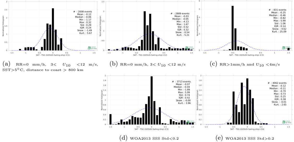
Figure 13: Normalized histogram of \Delta SSS (Aquarius SSS L2 OR v5 (NASA-GSFC) - TSG (GOSUD-Sailing-ship)) for 5 different subdatasets corresponding to: RR=0 mm/h, 3 < U_{10} < 12 m/s, SST >5^\circ C, distance to coast > 800 km (a), RR=0 mm/h, 3 < U_{10} < 12 m/s (b), RR >1 mm/h and U_{10} < 4 m/s (c), WOA2013 SSS Std <0.2 (d), WOA2013 SSS Std >0.2 (e).
