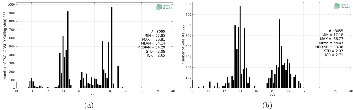
Figure 2: Histograms of SSS from TSG (GOSUD-Sailing-ship) (a) and Aquarius SSS L2 OR v5 (NASA-GSFC) (b) considering all match-up pairs per bins of 0.1 over the Equatorial Ocean 10N-10S Pi-MEP region and for the full satellite product period.
