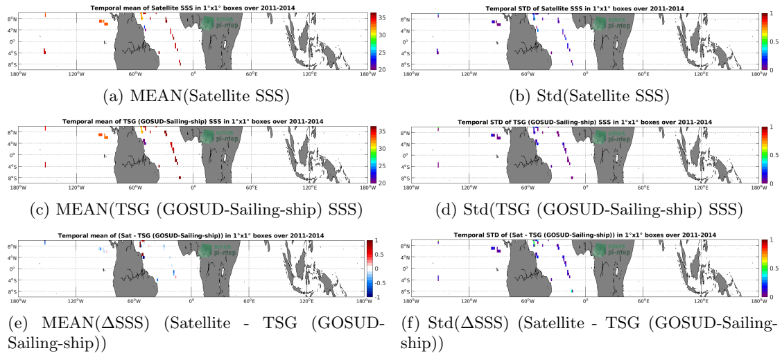
Figure 6: Temporal mean (left) and Std (right) of SSS from Aquarius SSS L2 OR v5 (NASA-GSFC) (top), TSG (GOSUD-Sailing-ship) (middle), and of \Delta SSS (Satellite - TSG (GOSUD-Sailing-ship)). Only match-up pairs are used to generate these maps.
