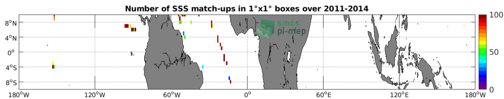
Figure 4: Number of SSS match-ups between TSG (GOSUD-Sailing-ship) SSS and the Aquarius SSS L2 OR v5 (NASA-GSFC) SSS product for the Equatorial Ocean 10N-10S Pi-MEP region over 1^\circ \times 1^\circ boxes and for the full satellite product period.
