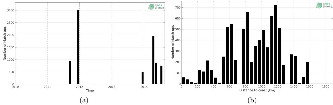
Figure 1: Number of match-ups between TSG (GOSUD-Sailing-ship) and Aquarius SSS L2 OR v5 (NASA-GSFC) SSS as a function of time (a) and as function of the distance to coast (b) over the Equatorial Ocean 10N-10S Pi-MEP region and for the full satellite product period.
